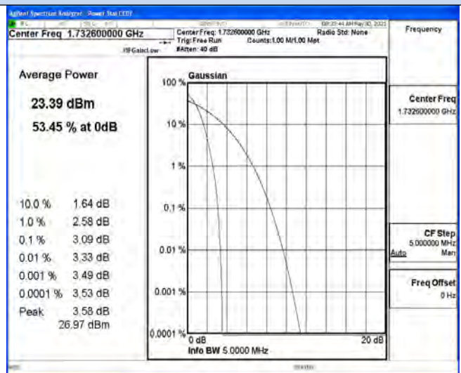
Channel 1413 / 1732.6 MHz
