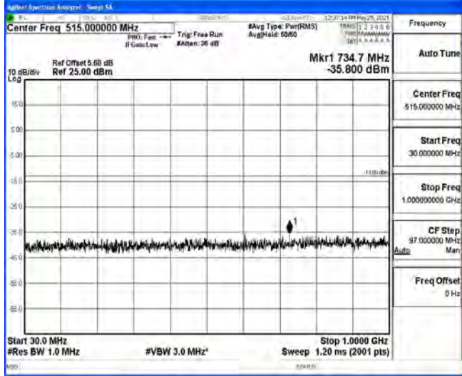
30 MHz – 1000 MHz
