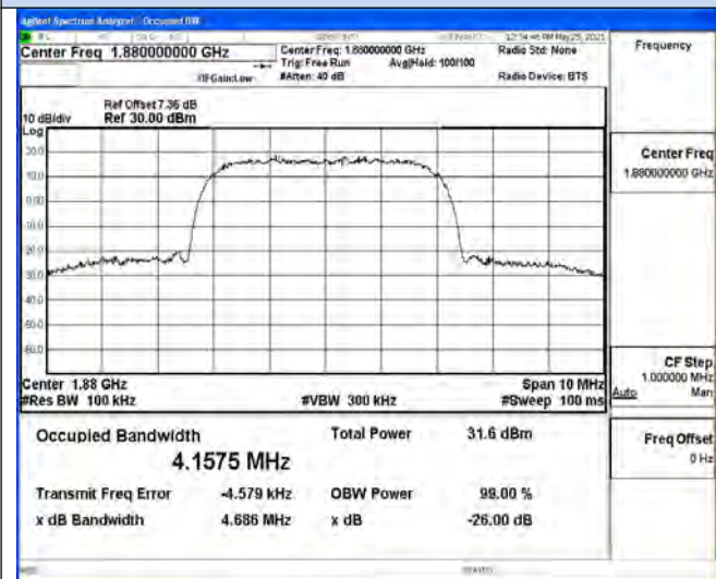
Channel 9400 / 1880.0 MHz
