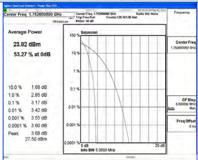
Channel 1513 / 1752.6 MHz
