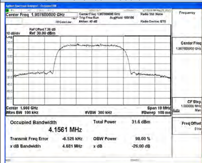
Channel 9538 / 1907.6 MHz
