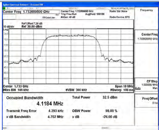
Channel 1413 / 1732.6 MHz
