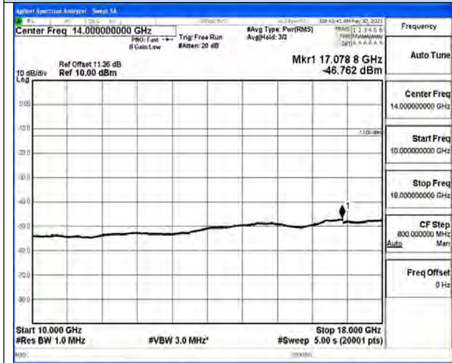
10 GHz – 18 GHz
