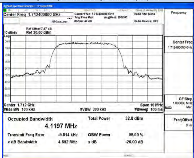
Channel 1312 / 1712.4 MHz
