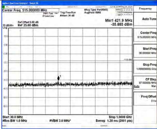
30 MHz – 1000 MHz
