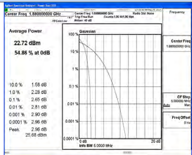
Channel 9400 / 1880.0 MHz
