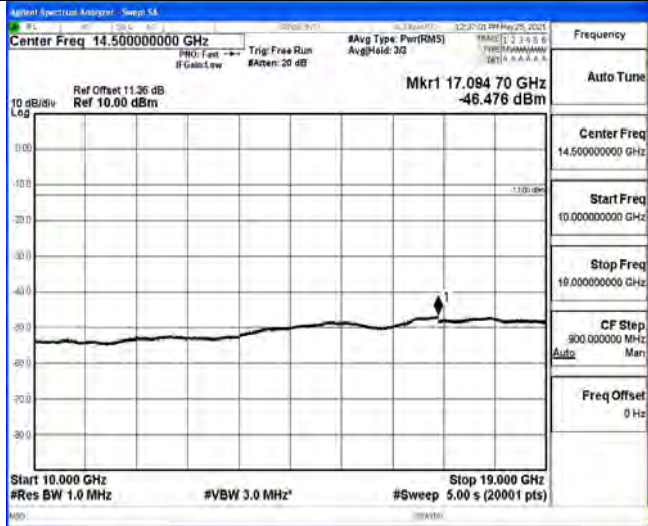
10 GHz – 19 GHz
