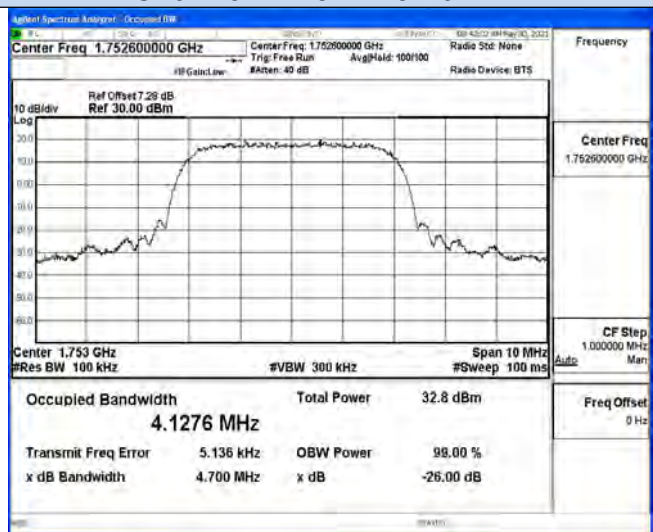
Channel 1513 / 1752.6 MHz
