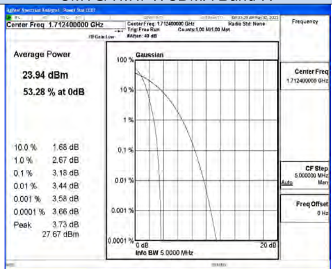
Channel 1312 / 1712.4 MHz
