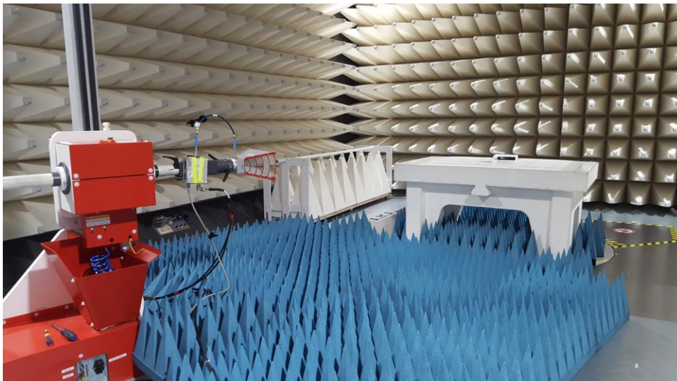
Figure B4. Hi Range Radiated Emission Set up
