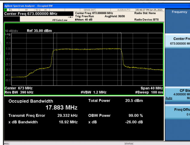
Band71-20MHz-16QAM-133322-100RB#0
