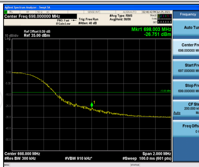
Band71-15MHz-16QAM-133197-75RB#0
