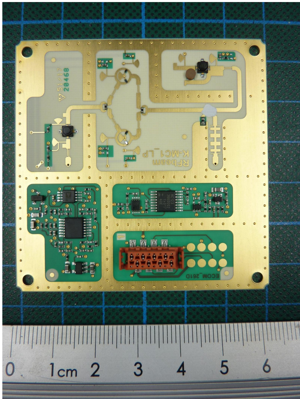
181708_i.jpg: K-MC1_LP, PCB, rear view
