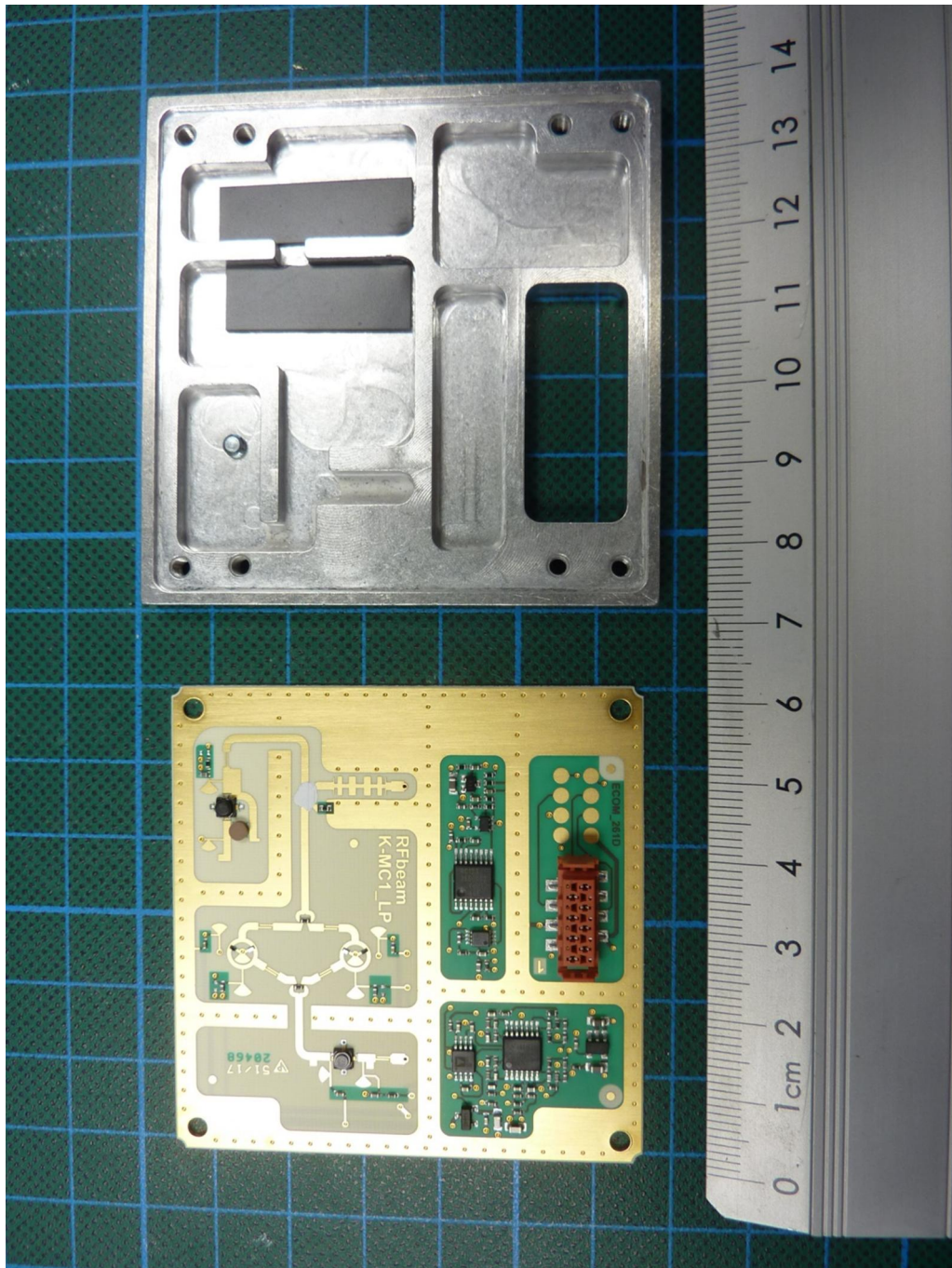
181708_h.jpg: K-MC1_LP, rear view (shielding removed)
