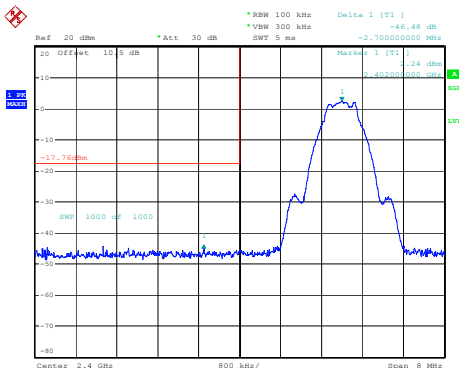
BLE_1M_Low_Channel
