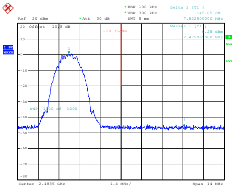
BLE_2M_High_Channel
