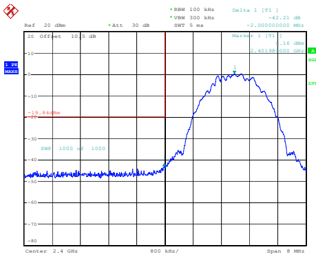
BLE_2M_Low_Channel
