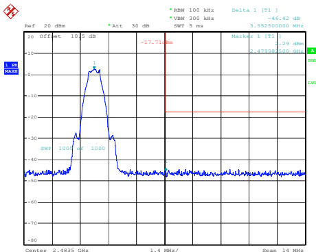
BLE_1M_High_Channel
