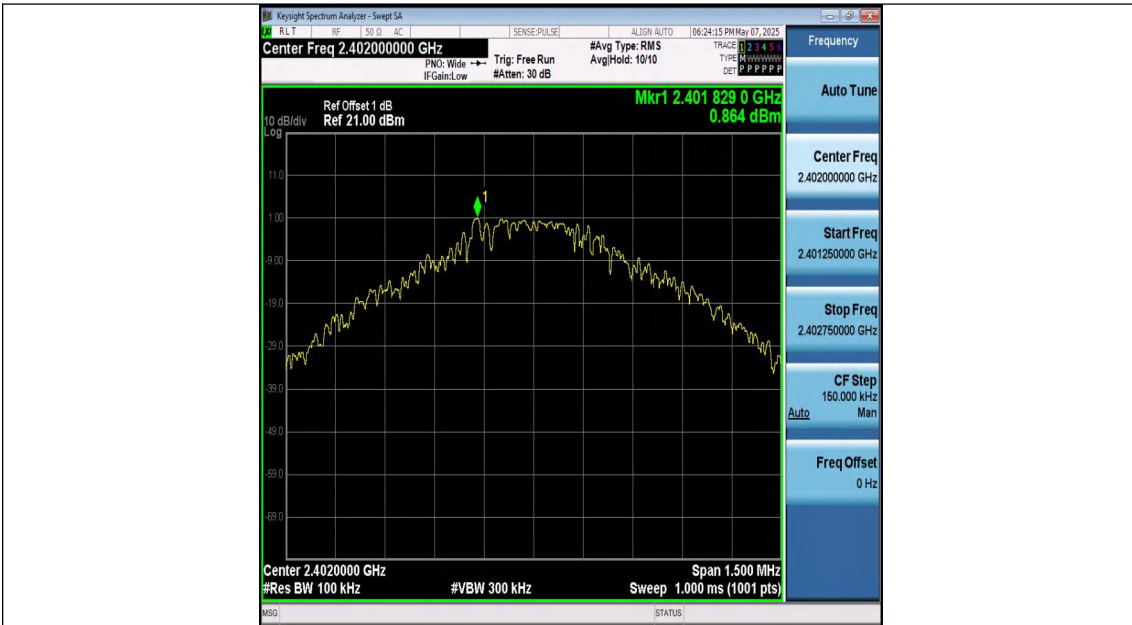
DH5-Ant1-2402-0~Reference-PASS
