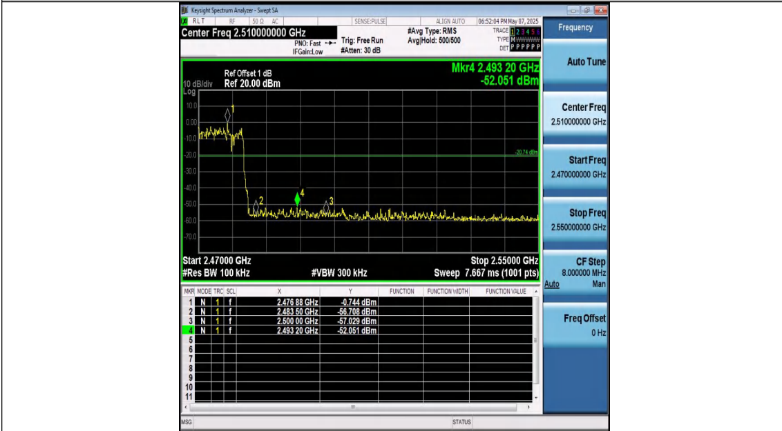
3DH5-Ant1-Hop_2480-PASS
