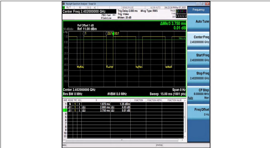
NTNV-DH5-Ant1-2402
