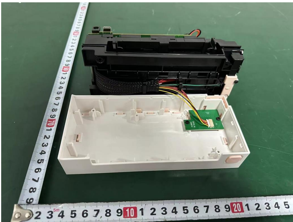
Internal photos M/N: PM-344-WF
