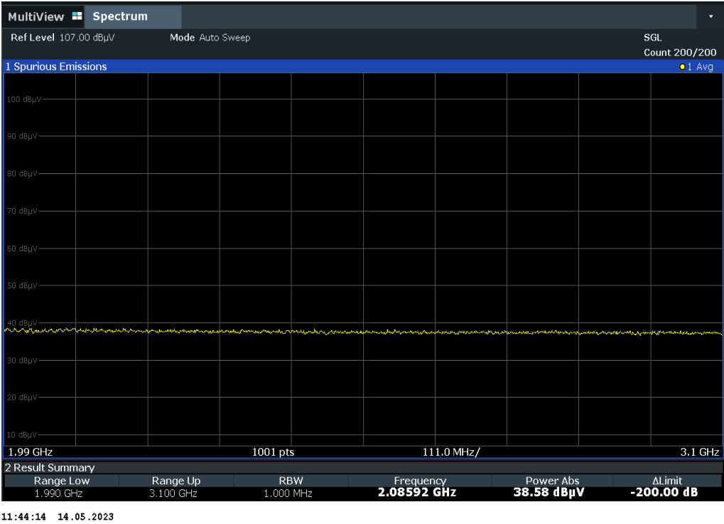
30.Spurious3-AV-CH9-H
