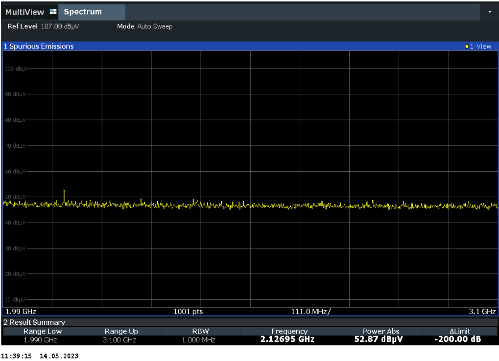
29.Spurious3-PEAK-CH9-H
