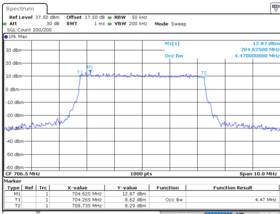
Occupied Bandwidth
