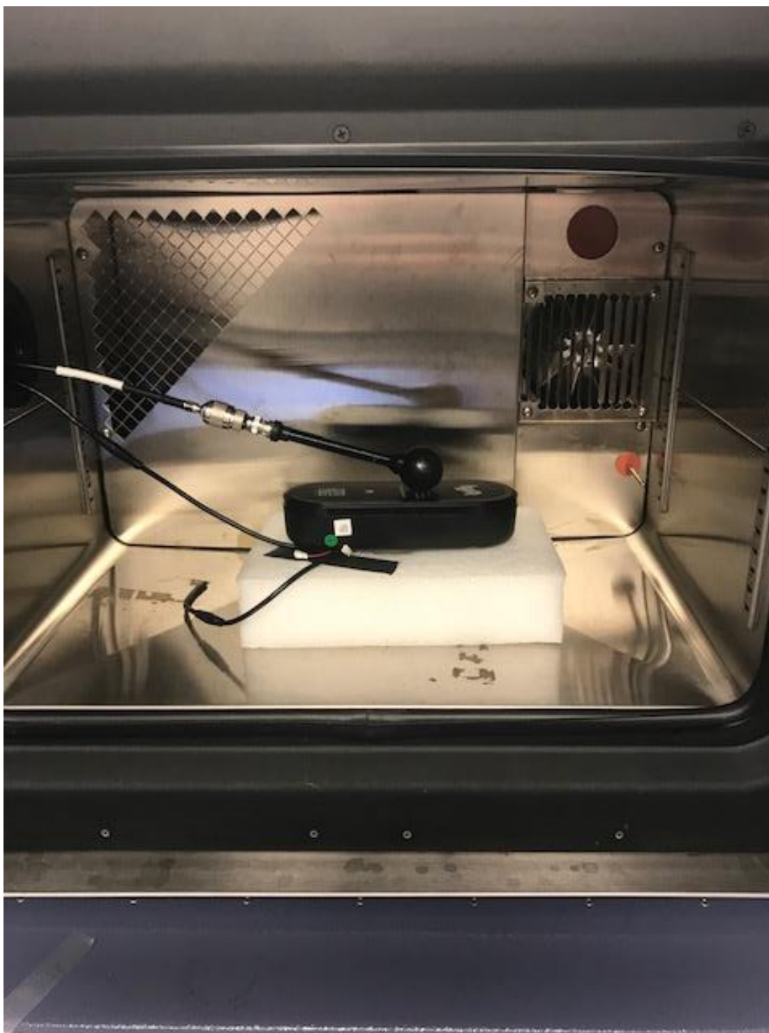
Test setup for Frequency Stability
