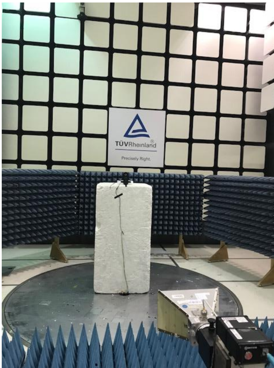
Test Setup 1-18G Front
