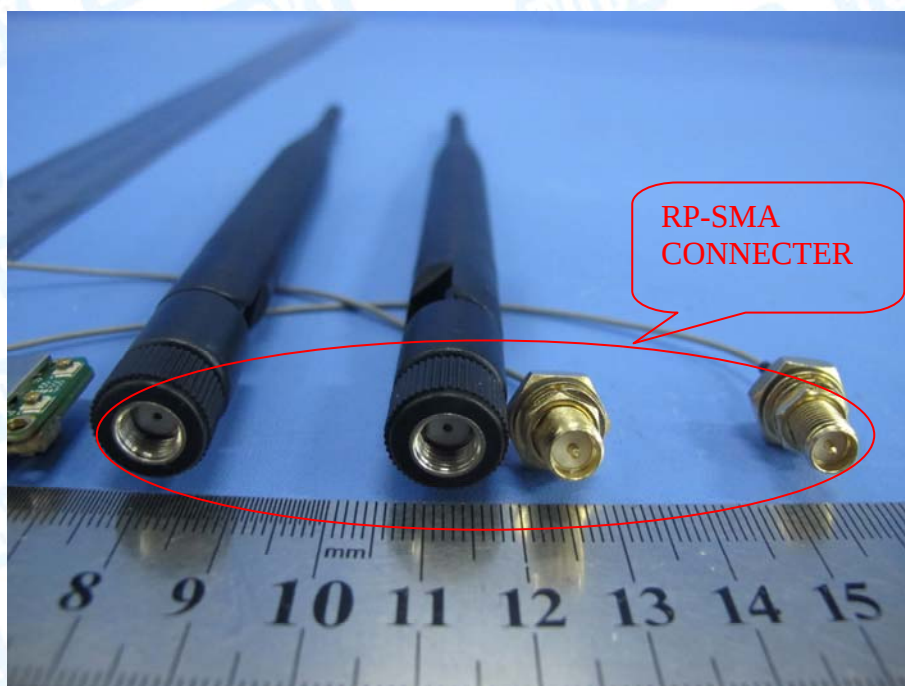
Photo 2 RF Connector Type
