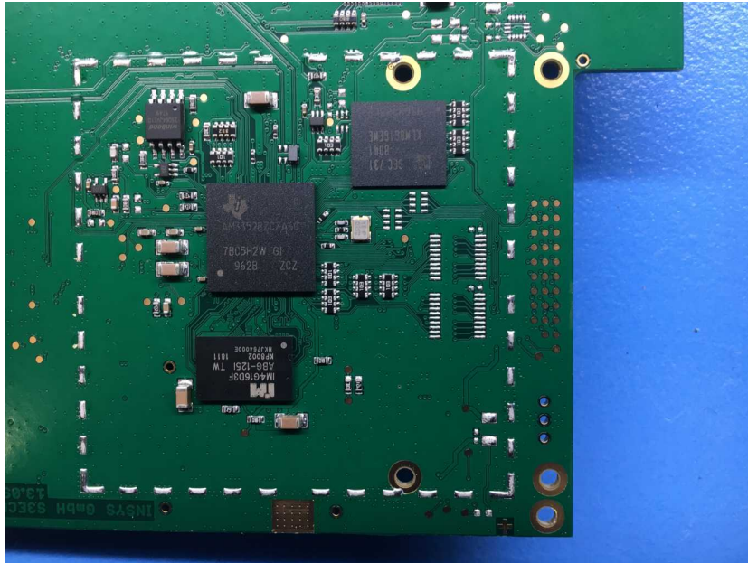
Photo 11: ECU board back side view with shielding removed
