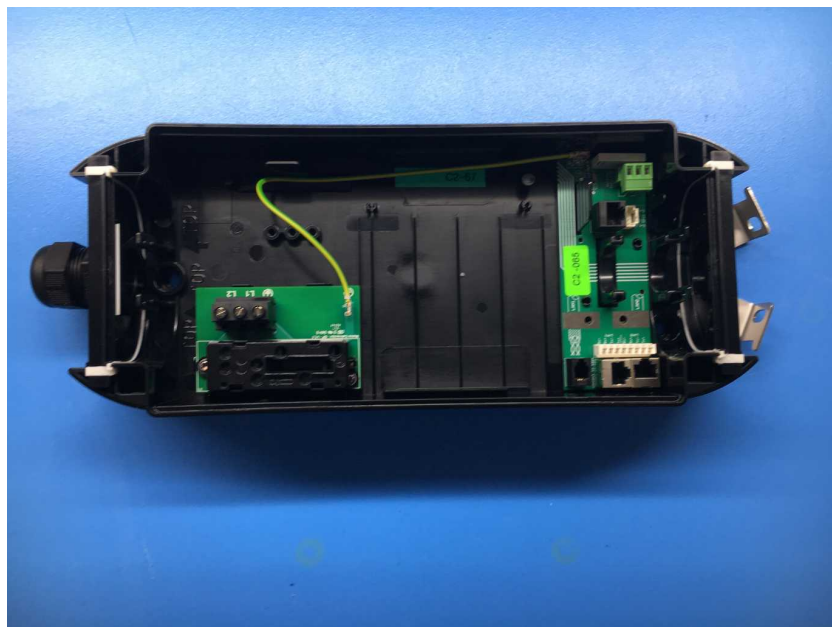
Photo 2: Casing front
