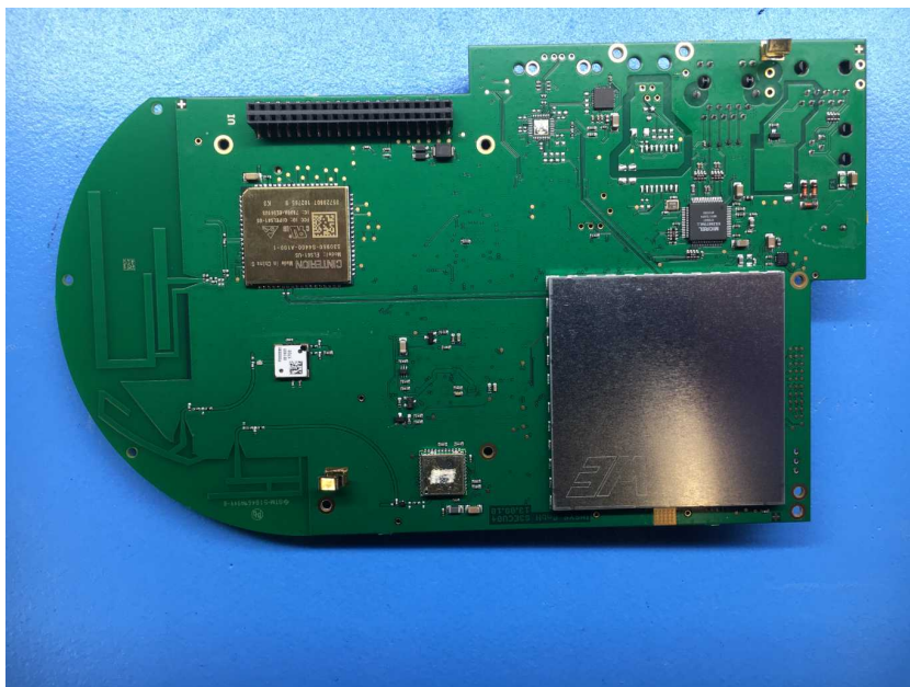
Photo 10: ECU board back side view with shielding
