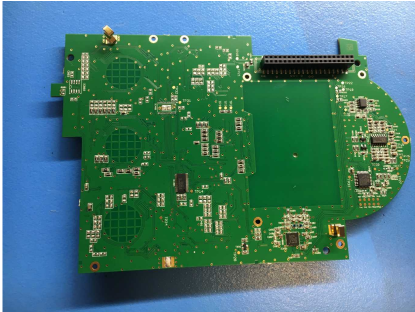
Photo 13: UI board back side view
