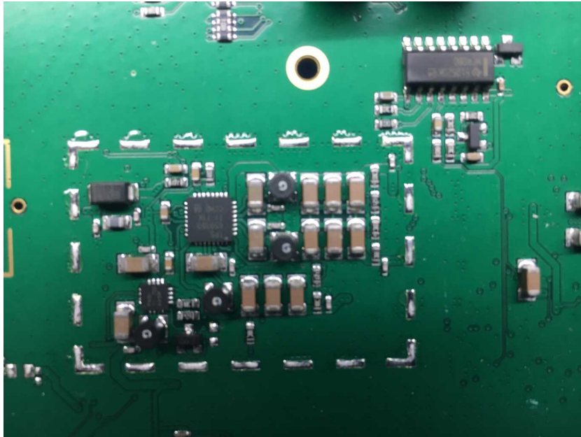
Photo 9: ECU board front side view with shielding removed
