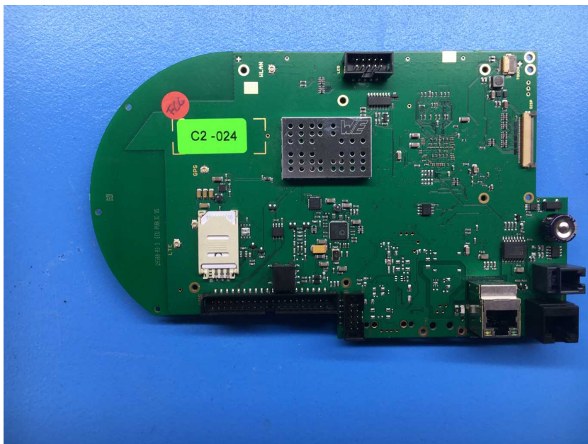
Photo 8: ECU board front side view with shielding
