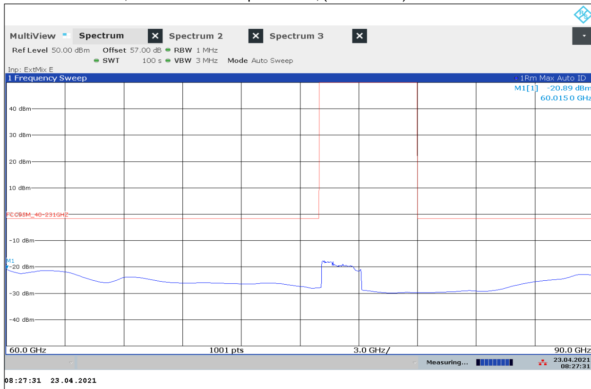
Plot 18: 60 GHz – 90 GHz, vertical / horizontal polarization, (mode5_4262)
