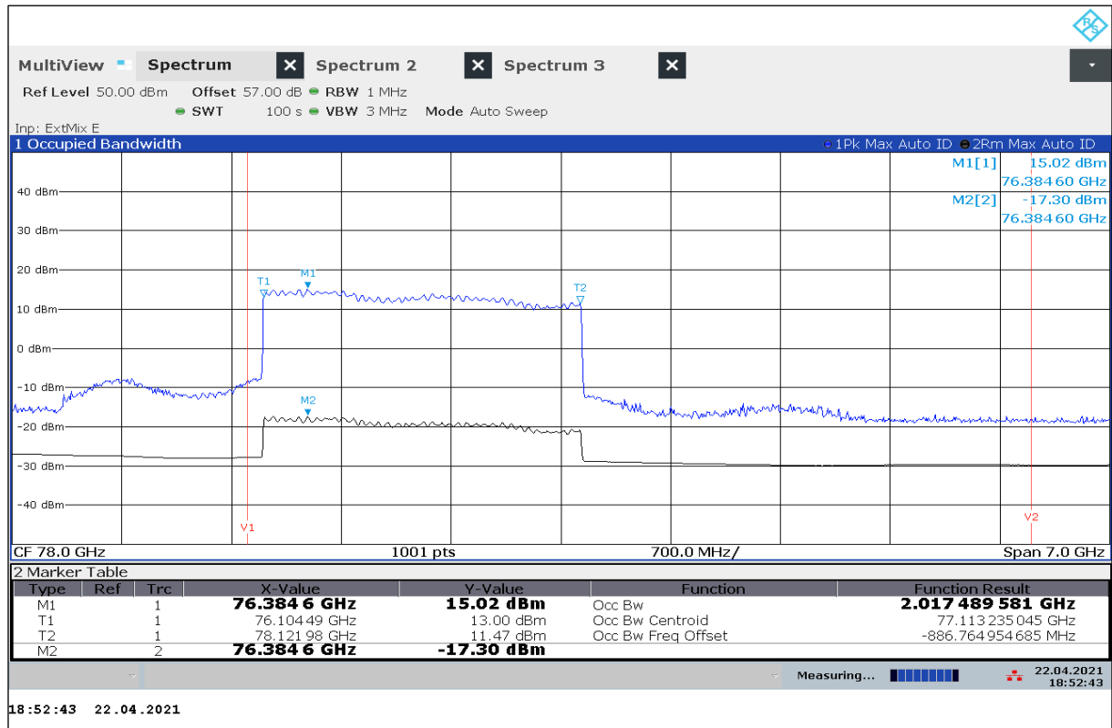
Plot 26: OBW, 20 °C / V min-max
