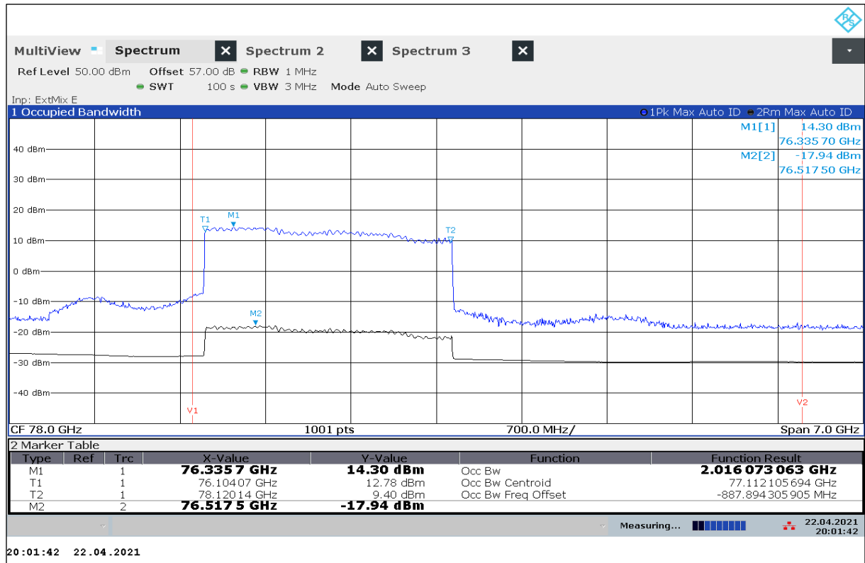
Plot 29: OBW, 50 °C / V_{min-max}
