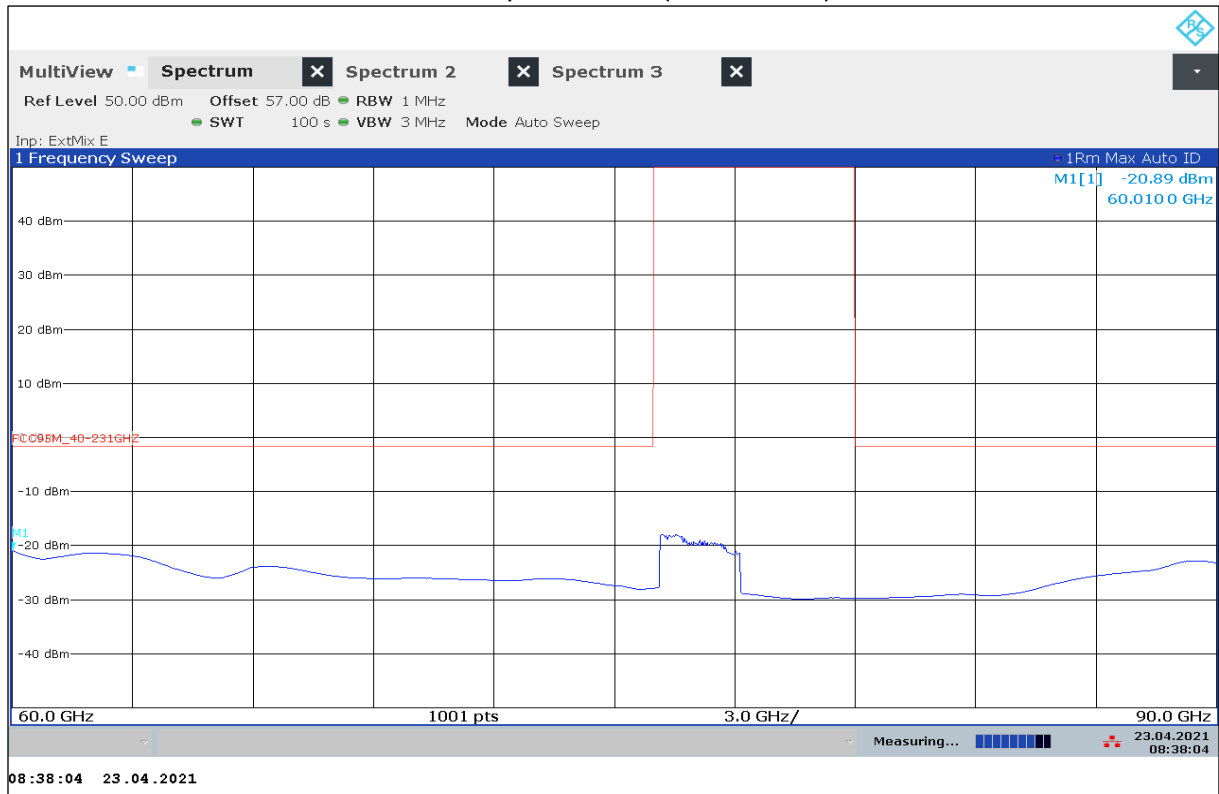
Plot 16: 60 GHz – 90 GHz, vertical / horizontal polarization, (mode5_5784)
