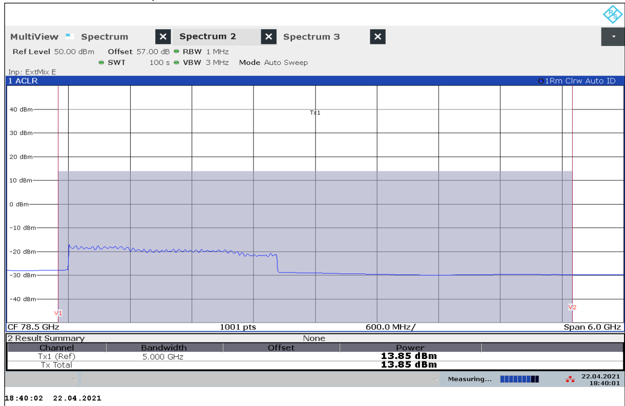
Plot 4: mode5_5784 – Mean power
