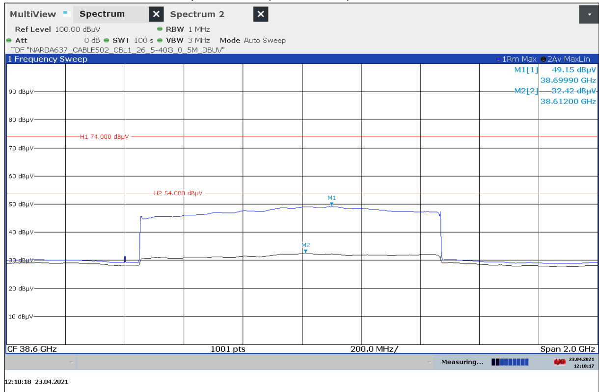
Plot 13: 38 GHz, vertical / horizontal polarization, (mode5_5169)
