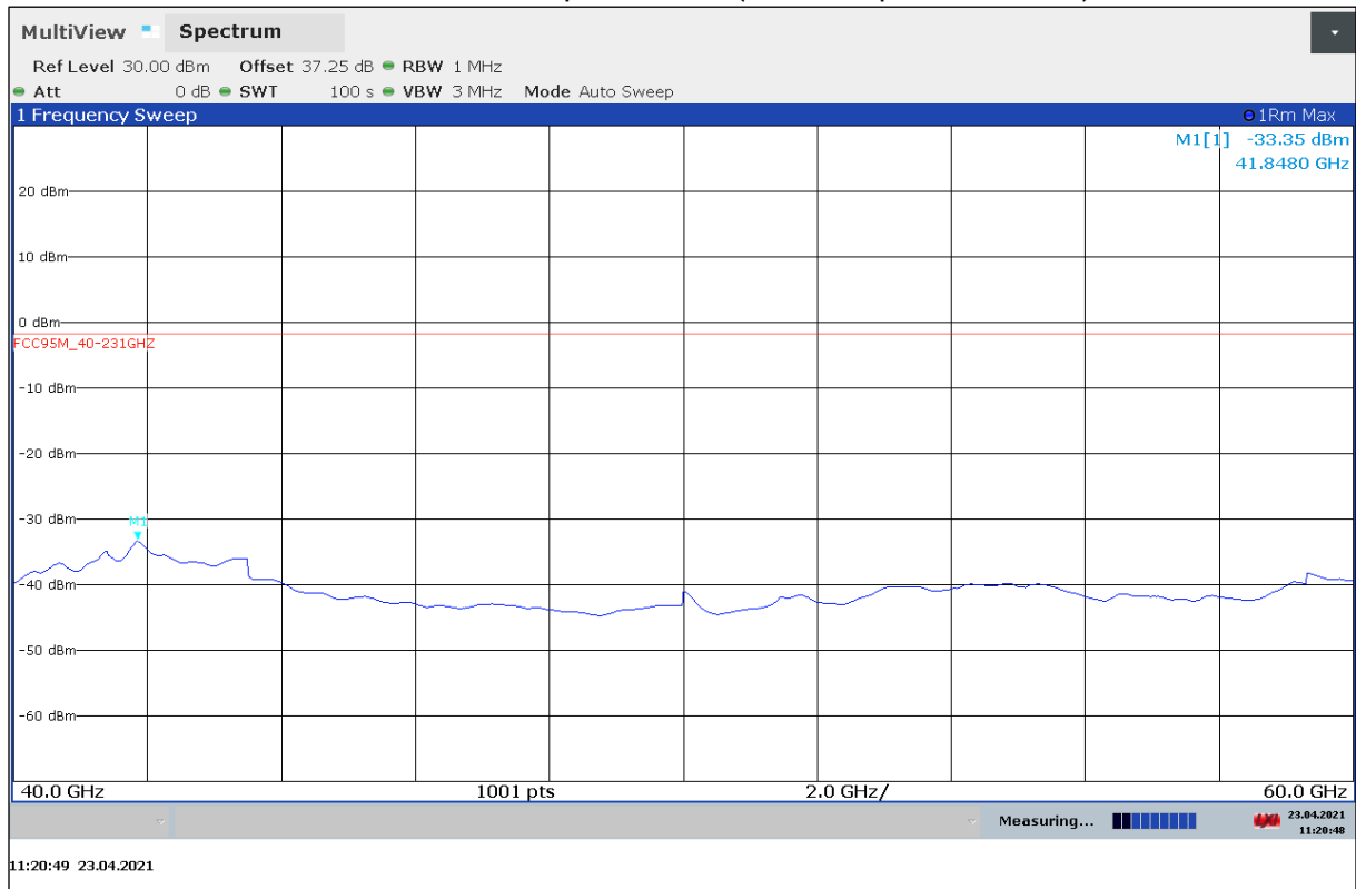
Plot 15: 40 GHz – 60 GHz, vertical / horizontal polarization, (Valid for specified Modes)
