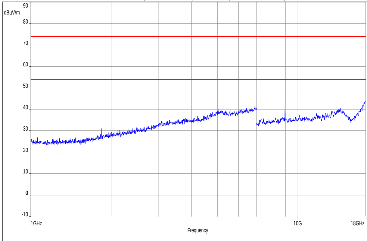
Plot 9: 1 GHz – 18 GHz, vertical / horizontal polarization, (Valid for specified Modes)
