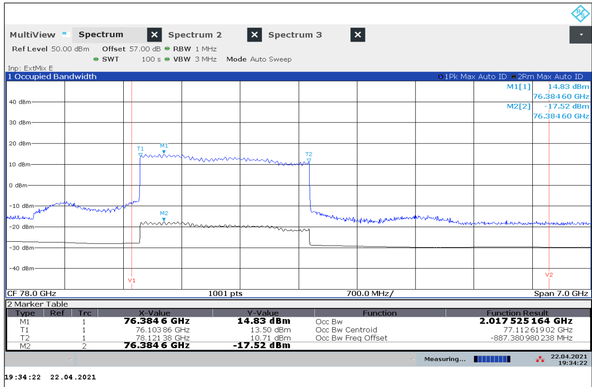
Plot 28: OBW, 40 °C / V_{nom}
