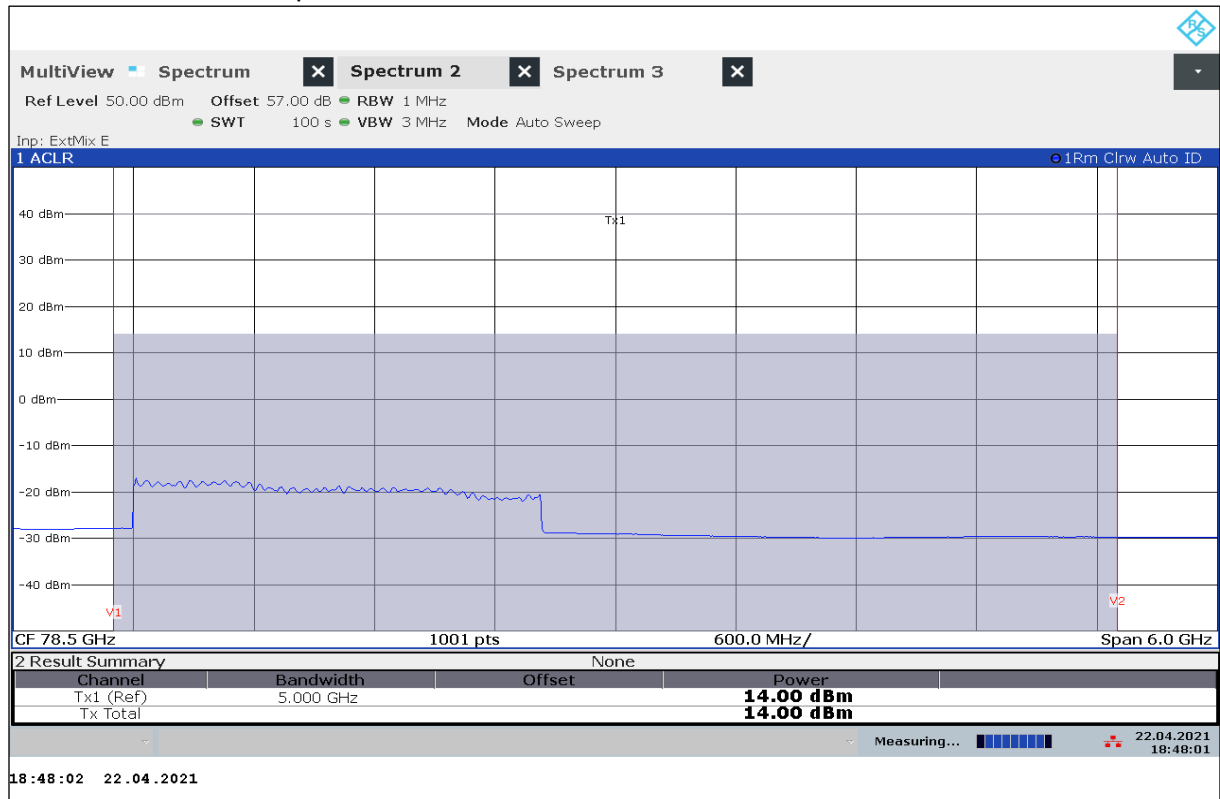
Plot 5: mode5_5169 – Mean power
