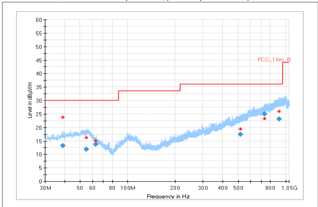
Plot 8: 30 MHz – 1 GHz, vertical / horizontal polarization, (Valid for specified Modes)
