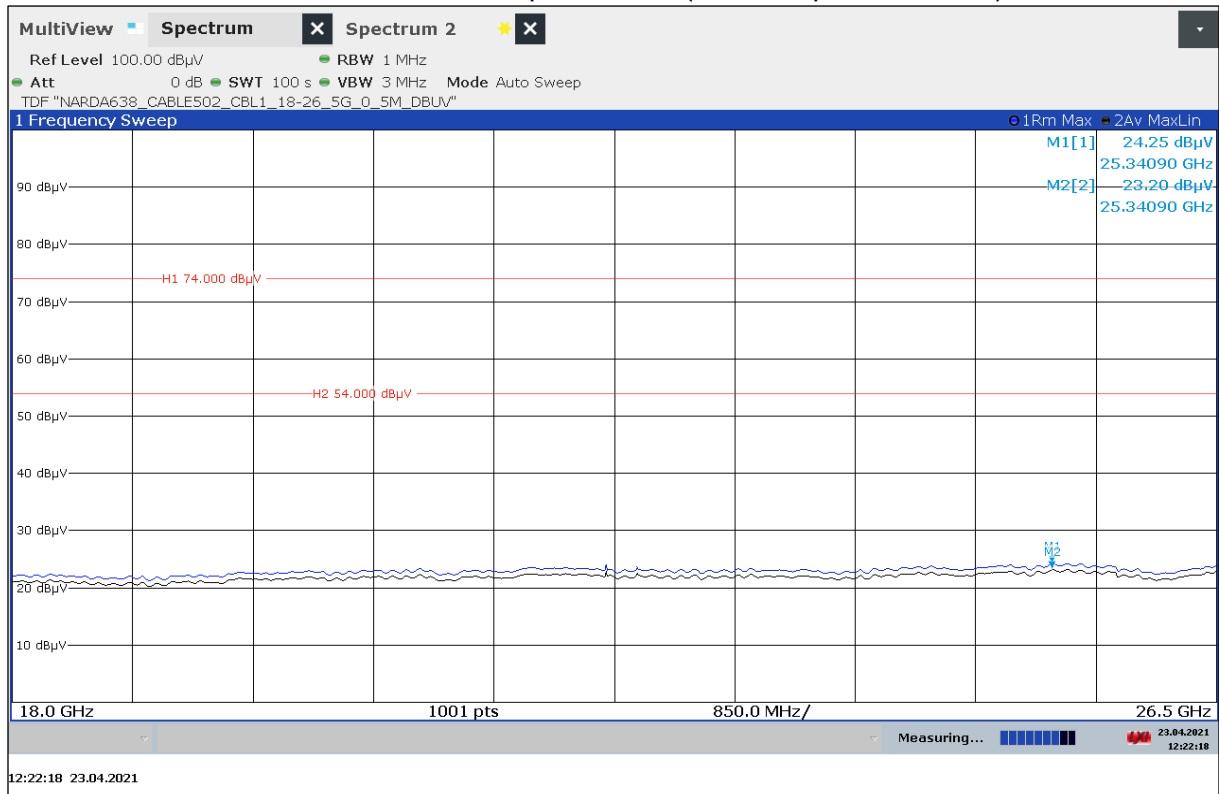
Plot 10: 18 GHz – 26.5 GHz, vertical / horizontal polarization, (Valid for specified Modes)
