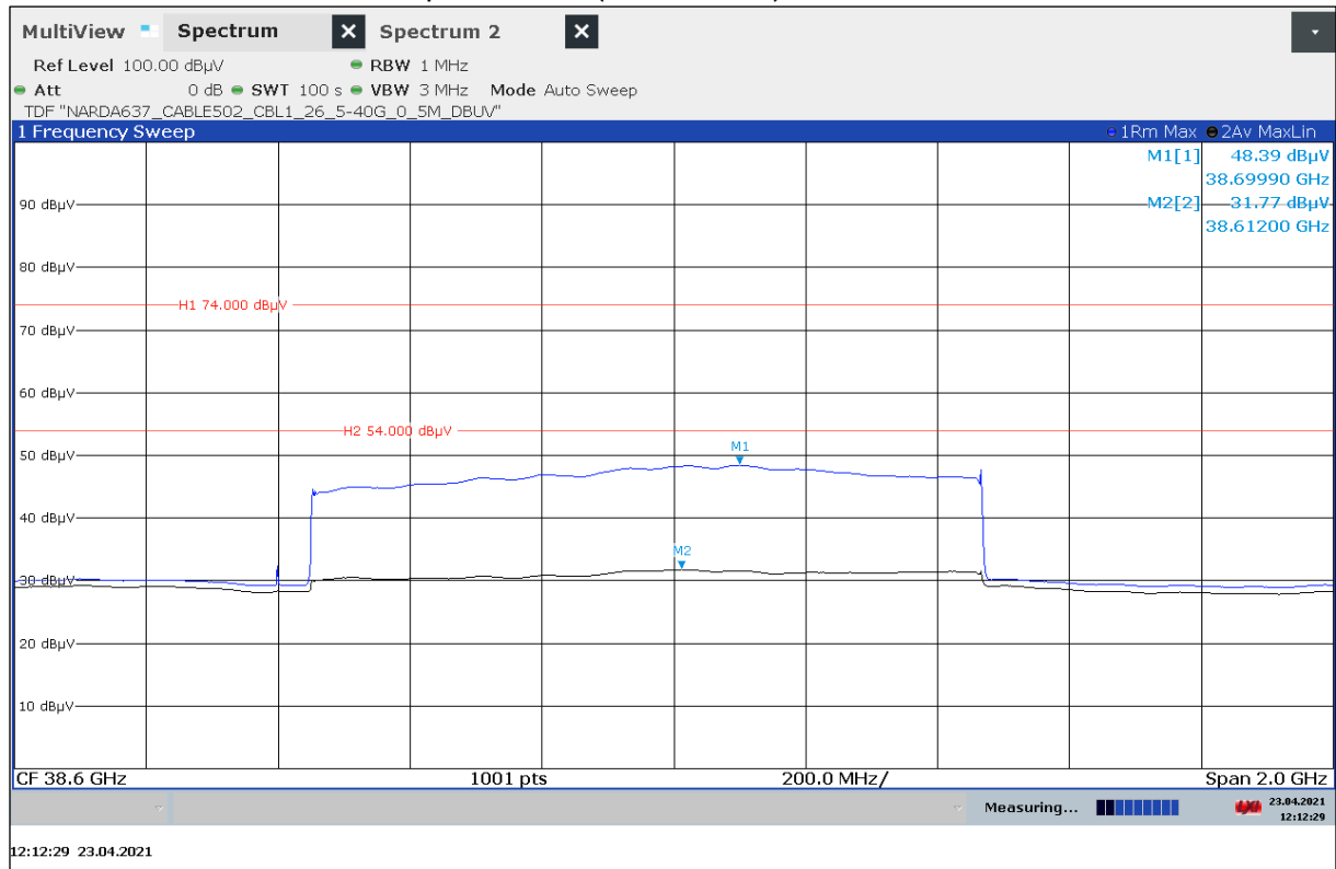
Plot 14: 38 GHz, vertical / horizontal polarization, (mode5_4262)
