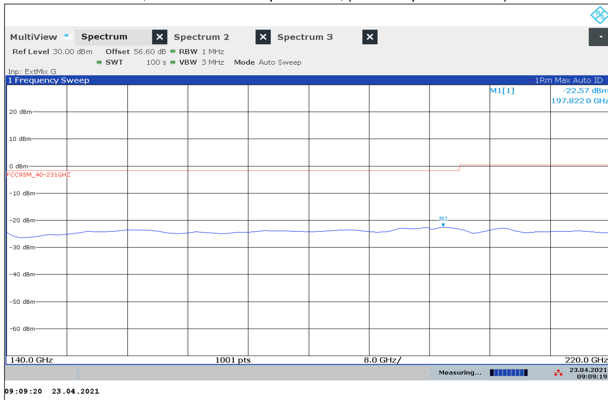
Plot 20: 140 GHz – 220 GHz, vertical / horizontal polarization, (Valid for specified Modes)
