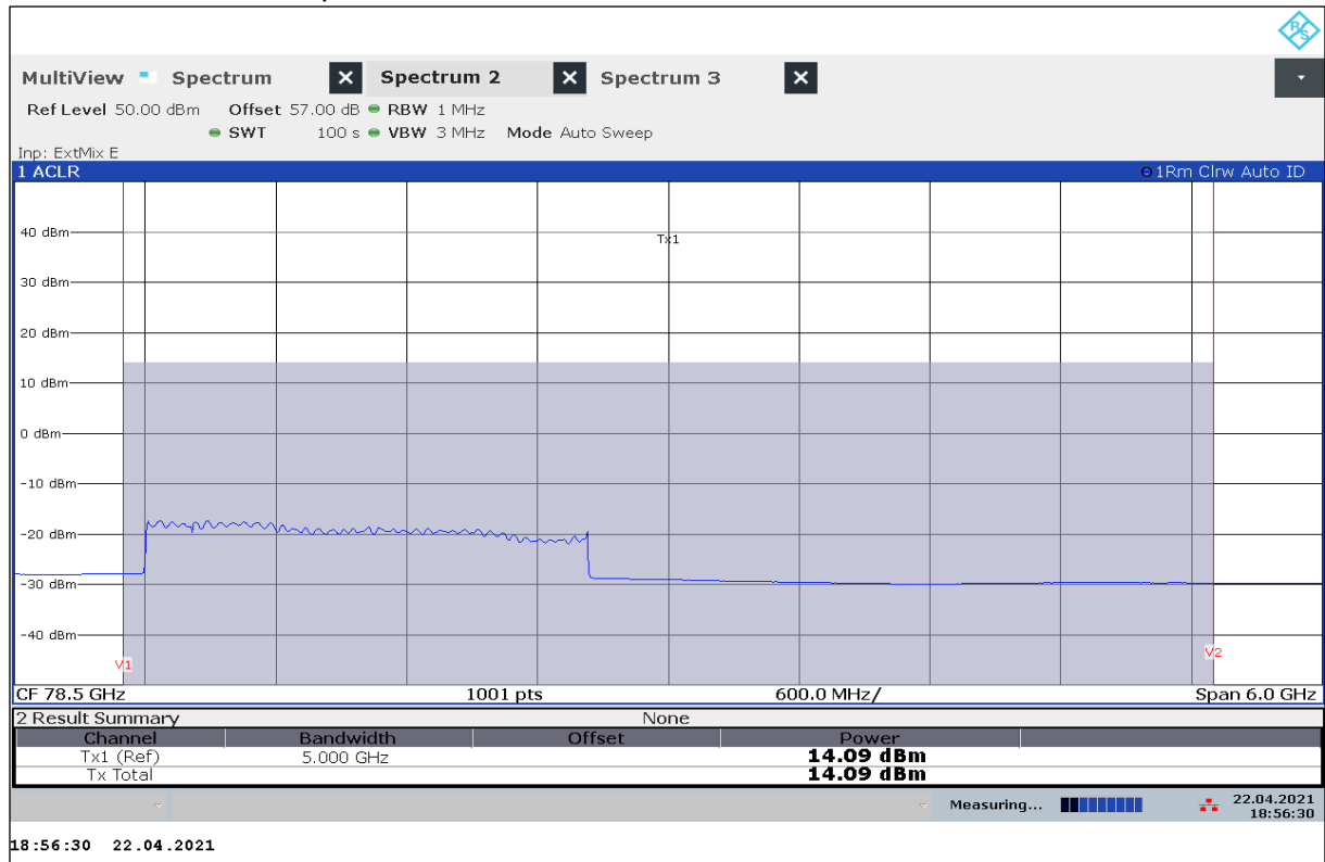
Plot 6: mode5_4262 – Mean power
