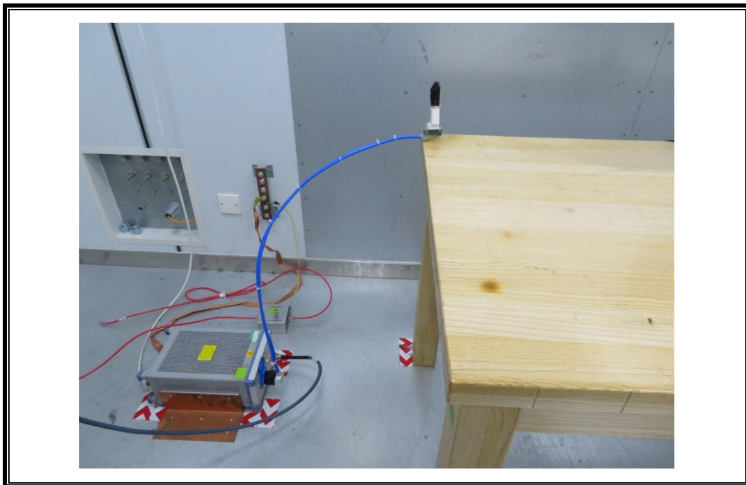
AC POWER LINE CONDUCTED EMISSIONS MEASUREMENT SETUP
