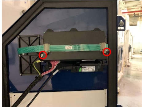
Figure 3: Module Installation
