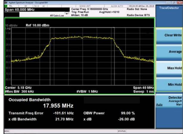
(802.11n20) -26dB&99% Bandwidth plot on channel 36
