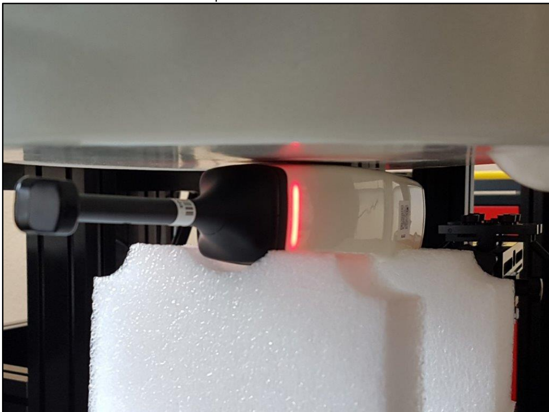
Photo 6: SAR test position - front side with 0 mm distance
