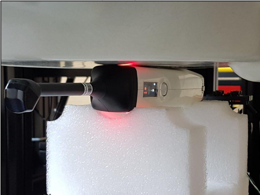
Photo 8: SAR test position - right side with 0 mm distance
