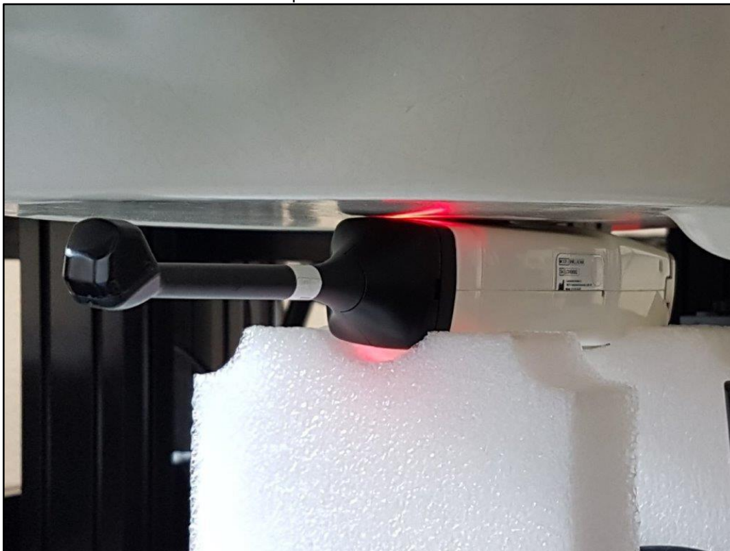
Photo 9: SAR test position – left side with 0 mm distance
