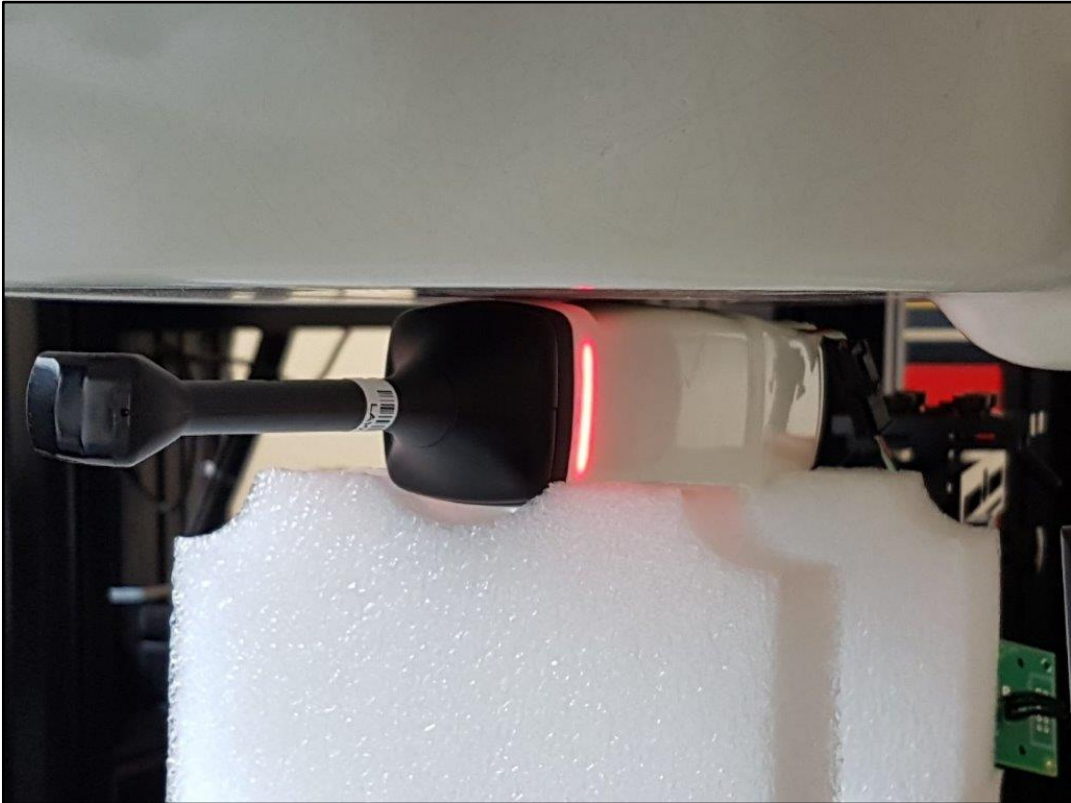
Photo 7: SAR test position - back side with 0 mm distance
