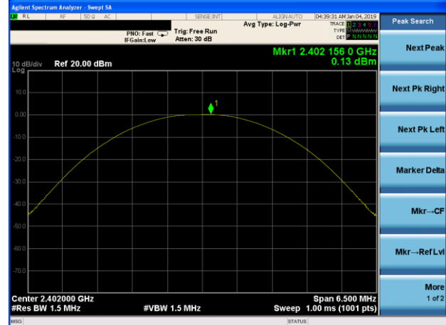
Peak output Power plot on channel 00 (2Mbps)
