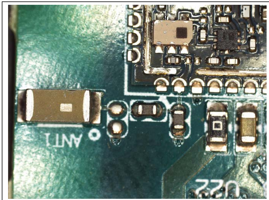
Radio Antenna
