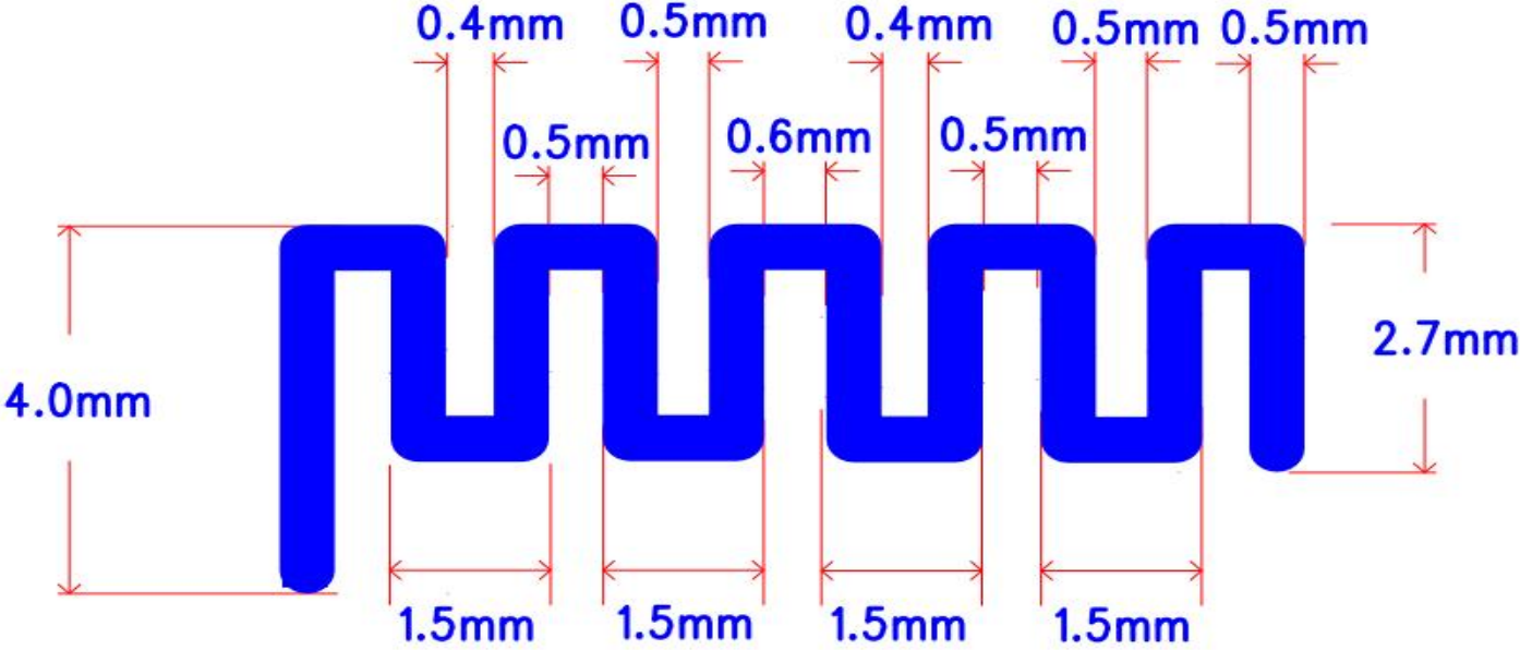
Antenna photo and length(mm)
