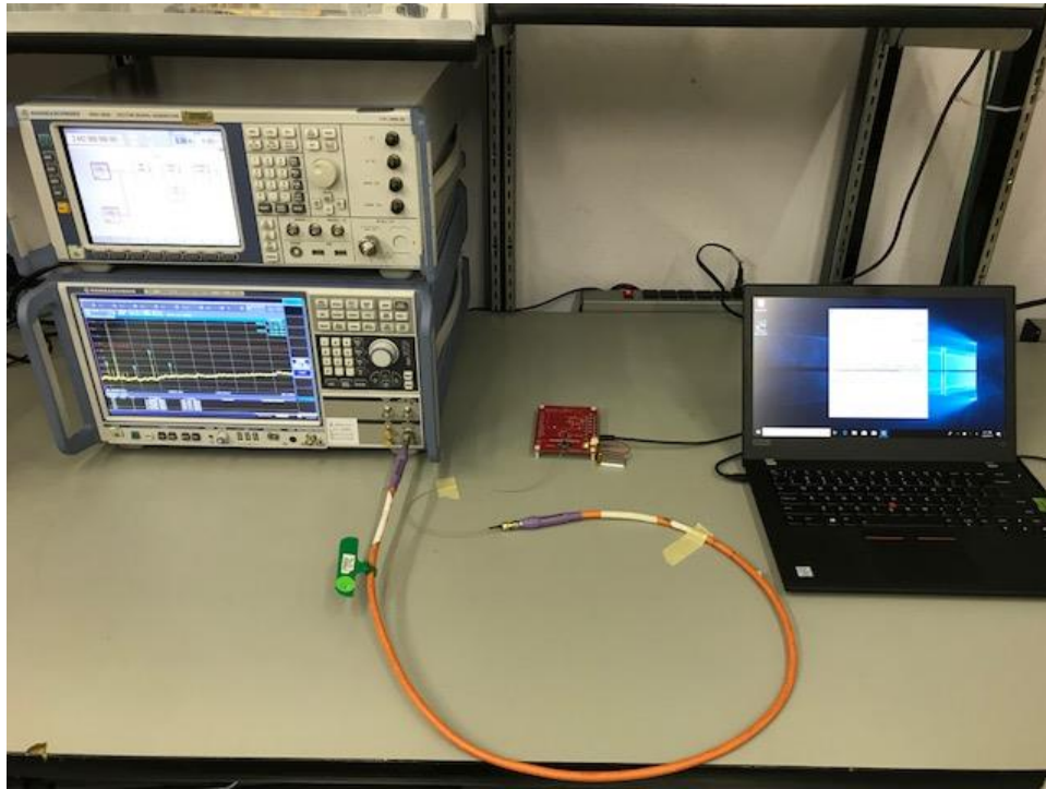
Figure 7: RF Conducted Test Setup
