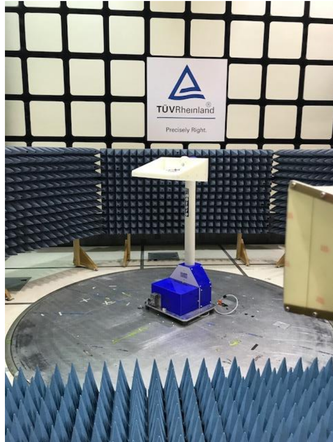
Figure 6: Test Setup for 1GHz to 18 GHz (Rear View)
