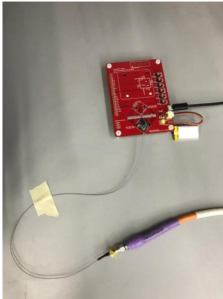
Figure 8: RF Conducted Test Setup (Detail)
