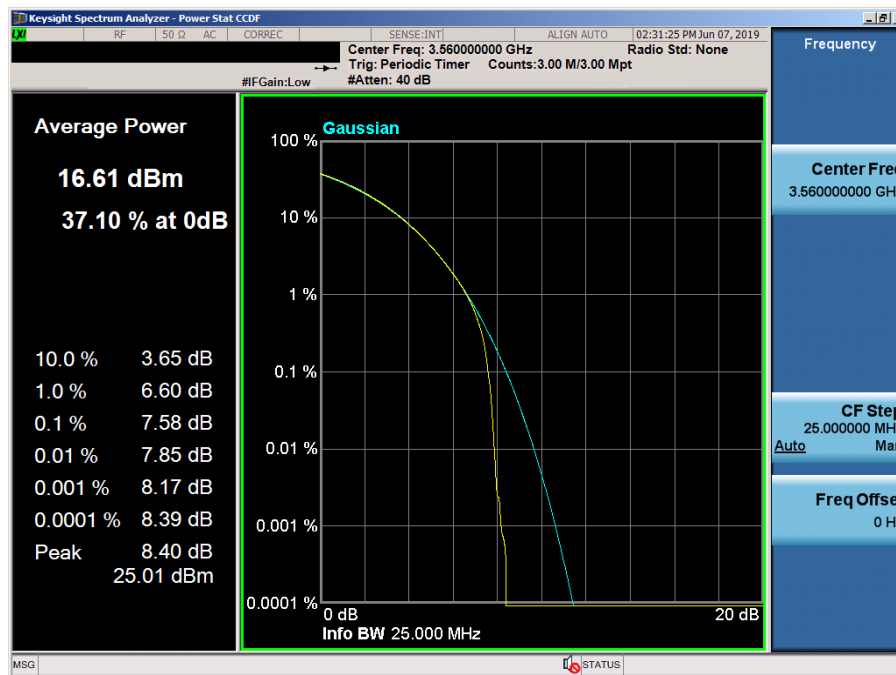
LTE Band 48 / 20 MHz / 16QAM
