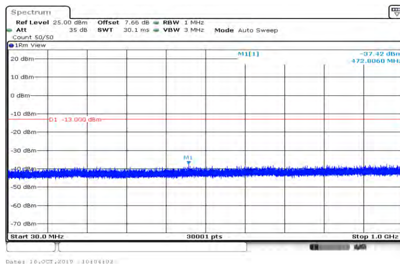
Band4-3MHz-16QAM-20175-1RB#0-Range1:30~1000MHz
