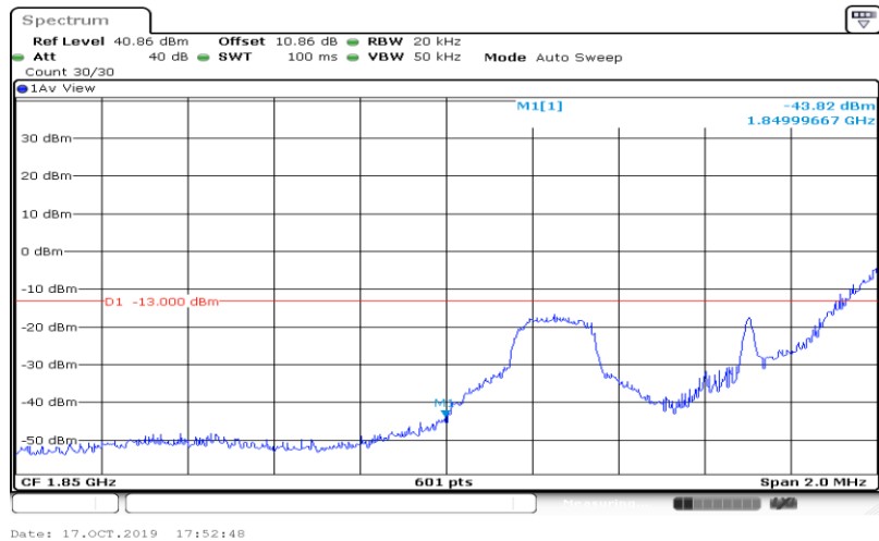
Band2-1.4MHz-QPSK-18607-6RB#0
