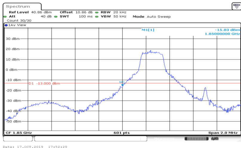
Band2-1.4MHz-QPSK-18607-1RB#5
