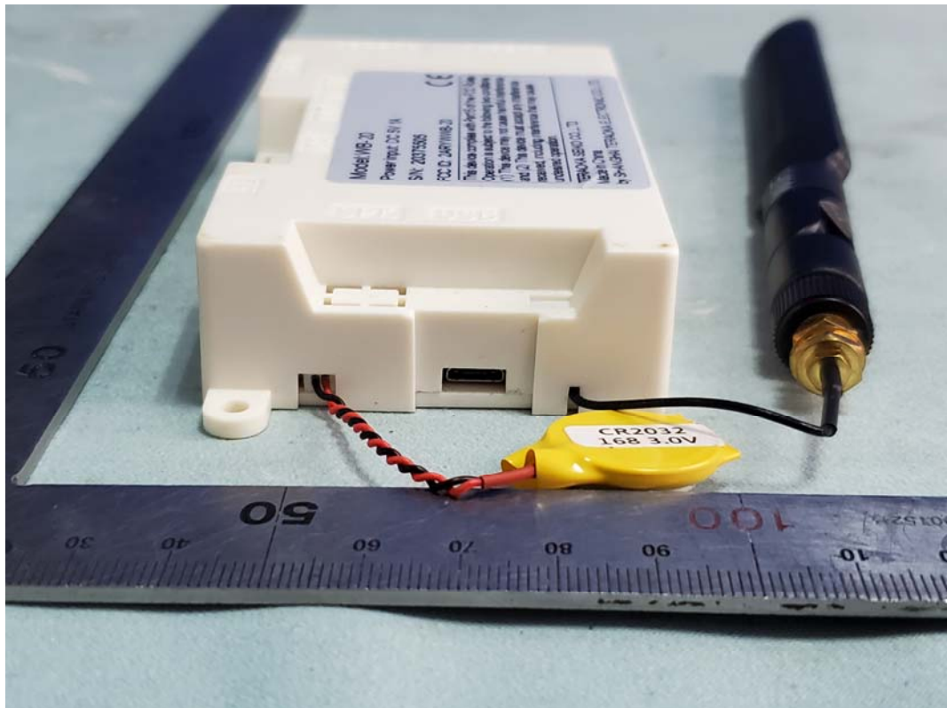
FIGURE 5 SMART CARD TERMINAL (M/N: WB-20) LEFT VIEW
