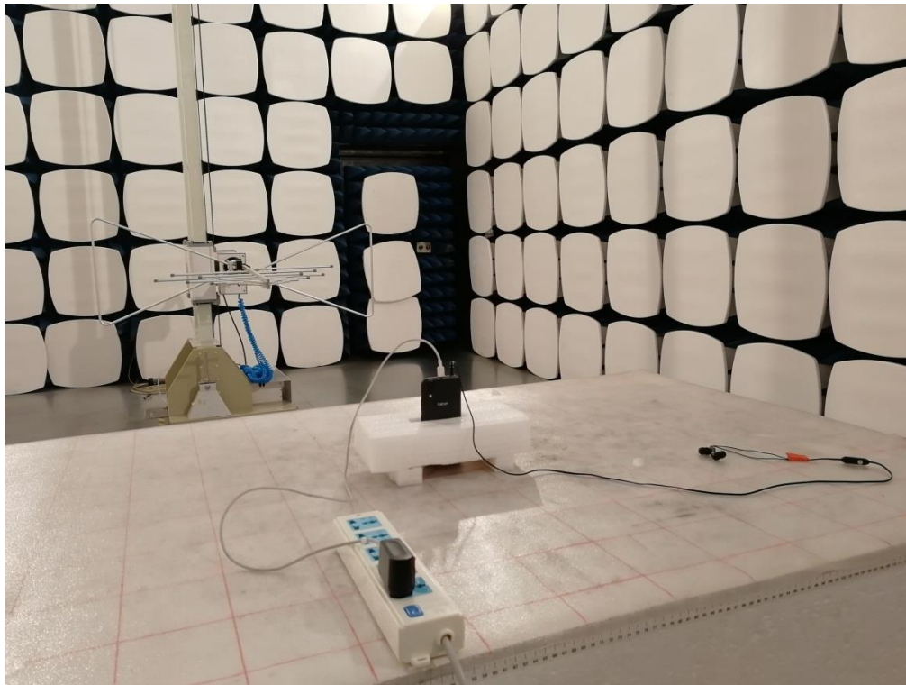
Radiated Spurious Emission UK Below 1GHz
