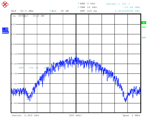
Low Channel -12.66dBm/3kHz
