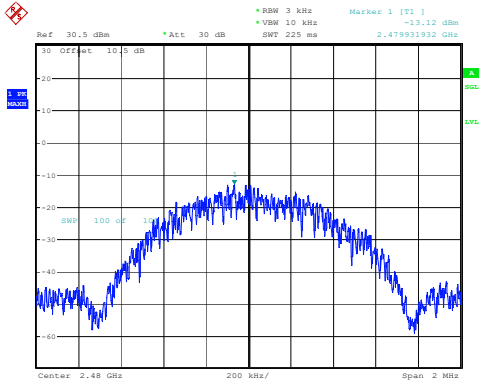
High Channel -13.12dBm/3kHz
