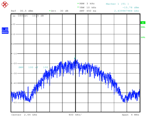
Middle Channel -15.78dBm/3kHz
