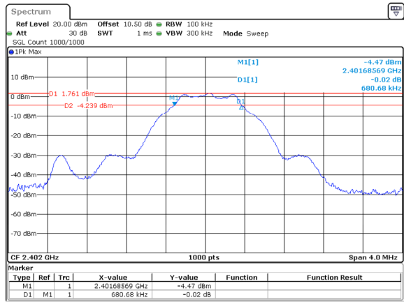
Low Channel 0.681MHz
