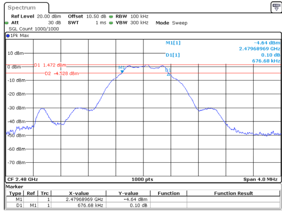
High Channel 0.677MHz
