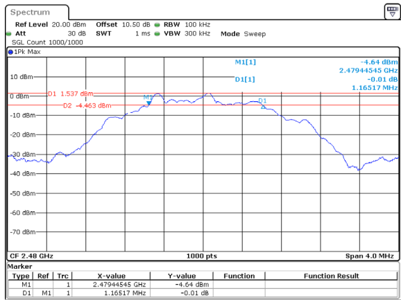
High Channel 1.165MHz
