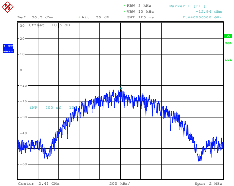
Middle Channel -12.94dBm/3kHz
