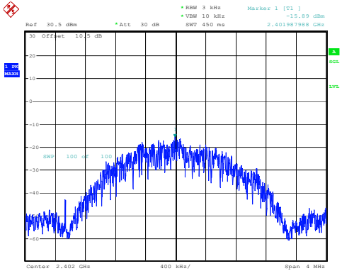
Low Channel -15.89dBm/3kHz
