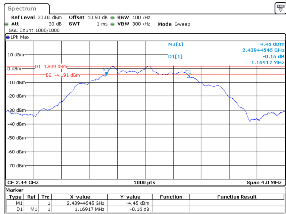
Middle Channel 1.169MHz
