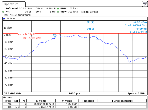
Low Channel 1.165MHz
