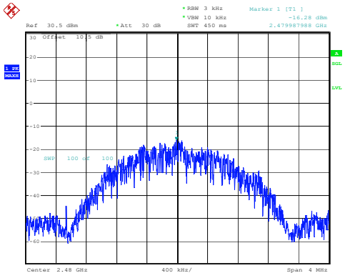
High Channel -16.28dBm/3kHz
