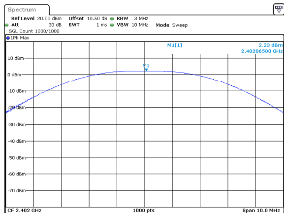
Low Channel 2.23dBm
