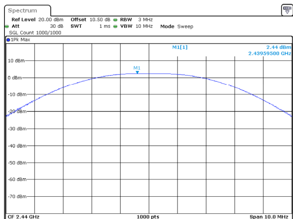
Middle Channel 2.44dBm
