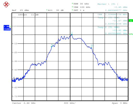
Middle Channel 1.029MHz
