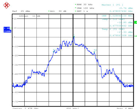
High Channel 2.029MHz
