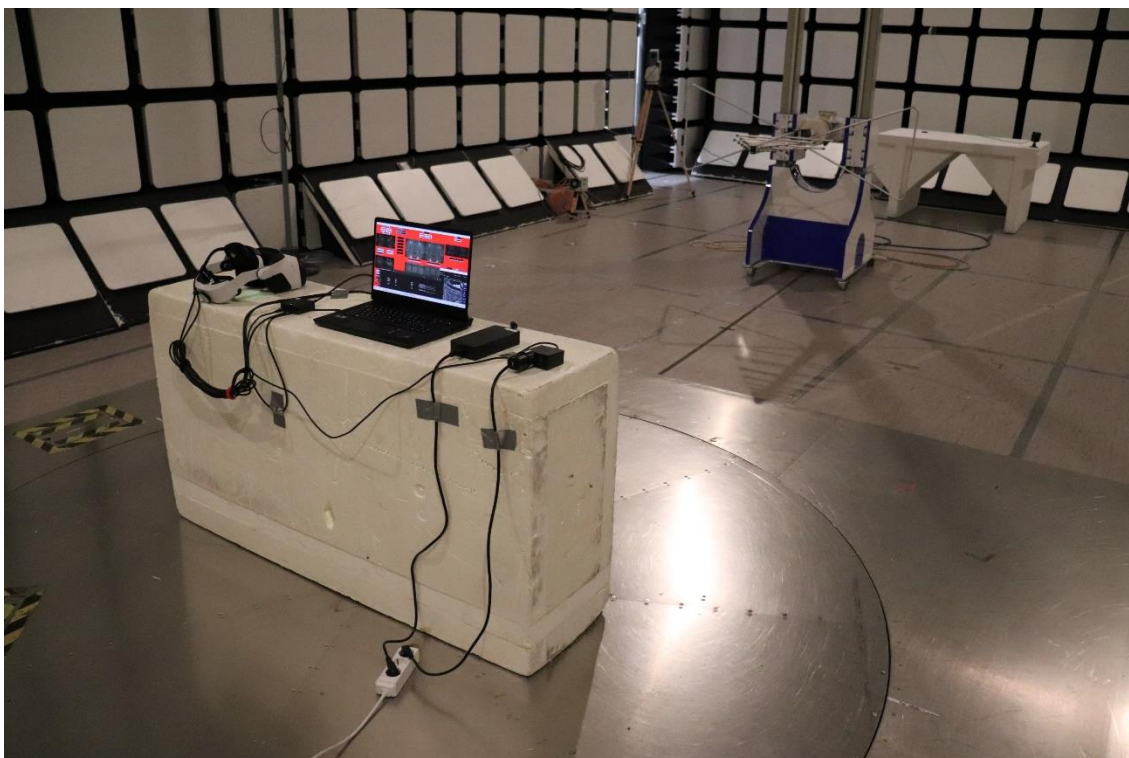
Photograph 3. Test setup for Radiated emissions 30 – 1000 MHz
