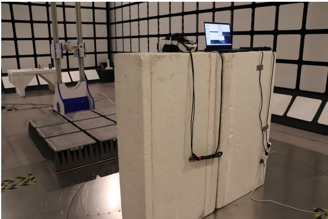
Photograph 5. Test setup for Radiated emissions 18 – 25 GHz
