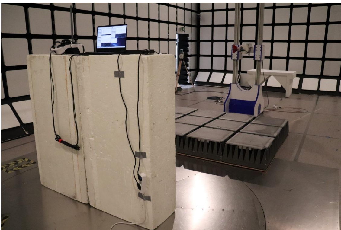
Photograph 4. Test setup for Radiated emissions 1 – 18 GHz
