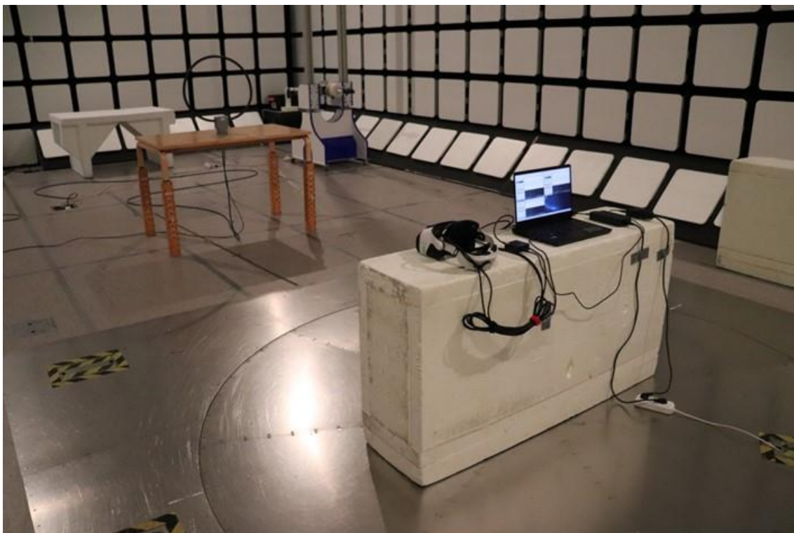
Photograph 2. Test setup for Radiated emissions 9 kHz – 30 MHz
