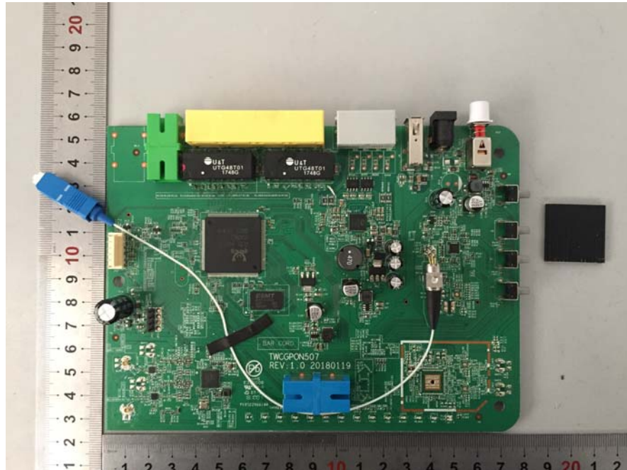
EUT – PCB-2 IC Chip View-1
