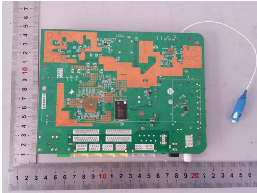
EUT – PCB-2 IC Chip View-2
