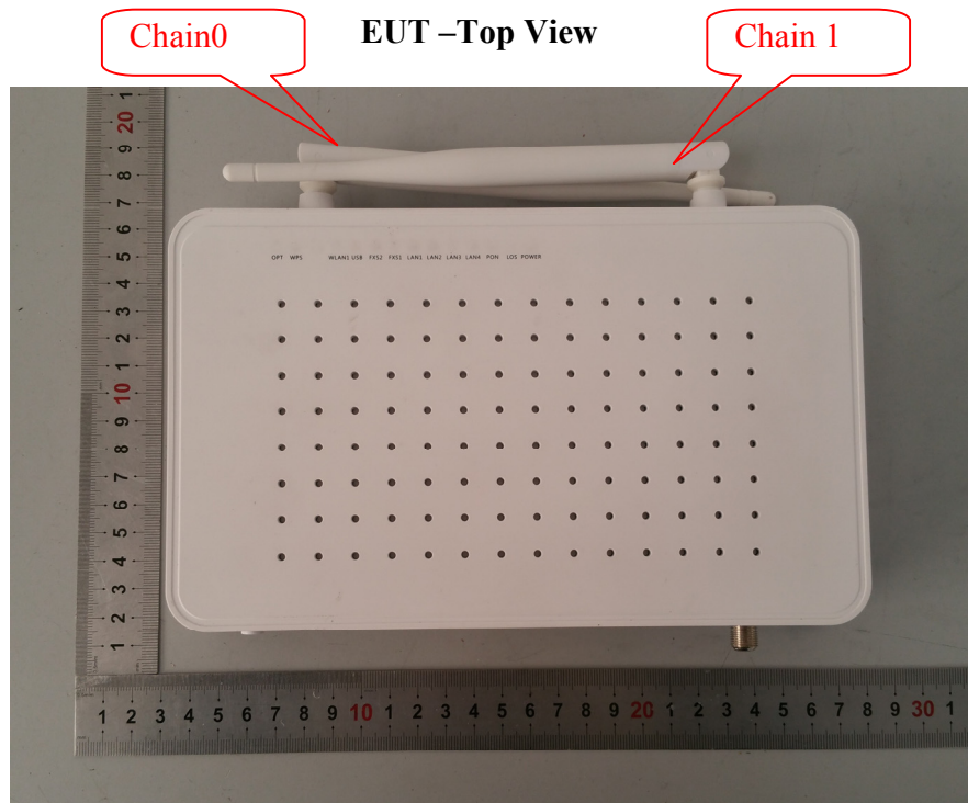
BDCOM GP1704-4GVC-S
