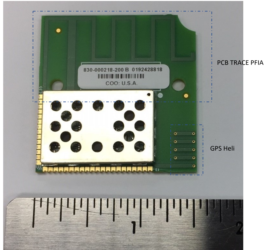
Figure 1. WLoRa Module, Top Side
