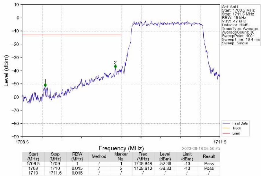
Band4_1.4MHz_QPSK_LCH_1710.7MHz_RB_6_0_NTNV
