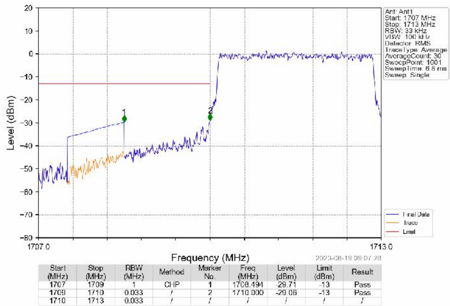
Band4_3MHz_QPSK_LCH_1711.5MHz_RB_15_0_NTNV
