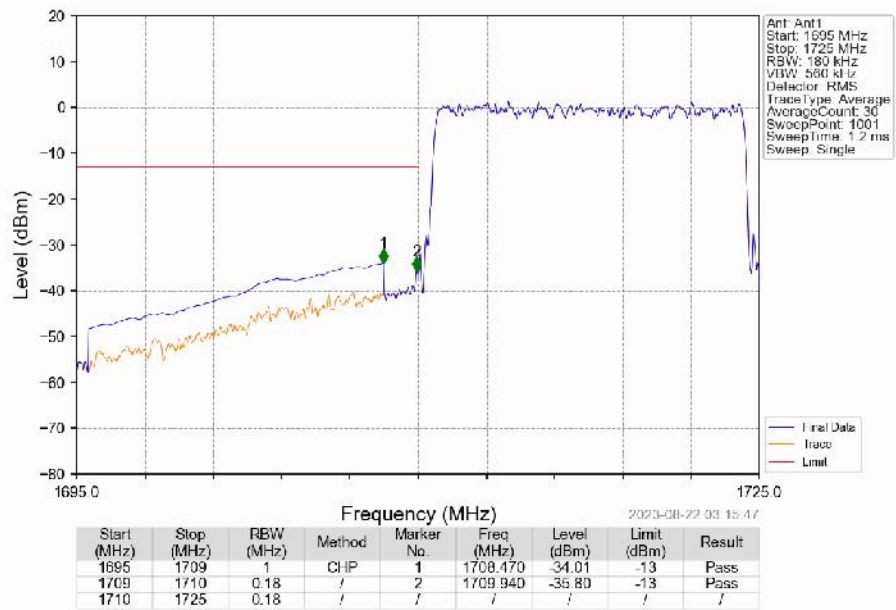
Band4_15MHz_QPSK_LCH_1717.5MHz_RB_75_0_NTNV
