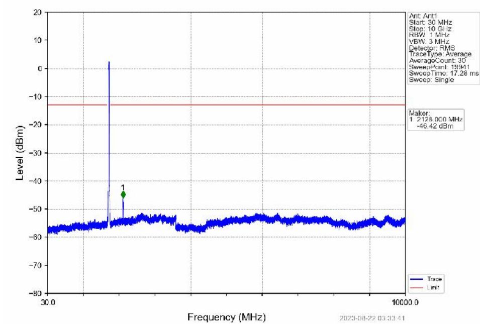
Band4_20MHz_16QAM_MCH_1732.5MHz_RB_1_0_NTNV
