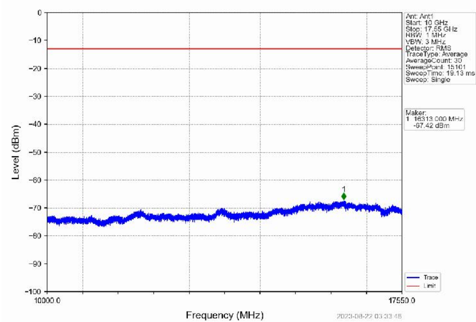
Band4_20MHz_16QAM_MCH_1732.5MHz_RB_1_0_NTNV
