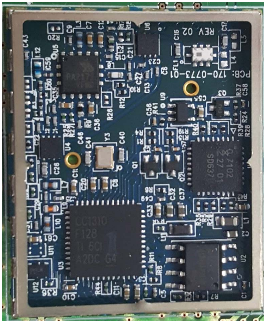
Radio PCB with Shield removed
