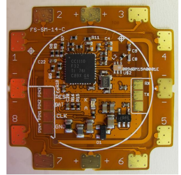
Sensor floor SF-LR (left), SF-HR (middle) and the Wireless Sensor Board SM14C (right)
