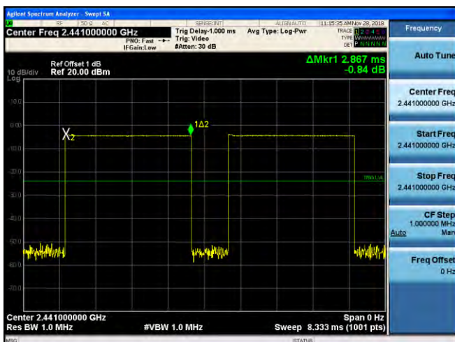
Middle Channel / 2441 MHz - DH5
