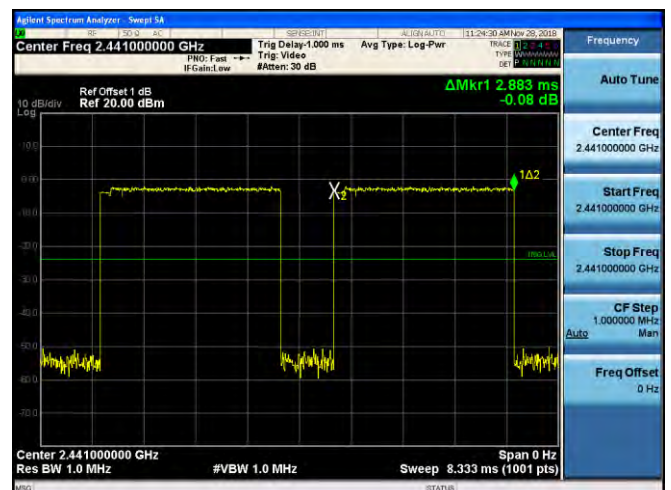
Middle Channel / 2441 MHz - 2DH5
