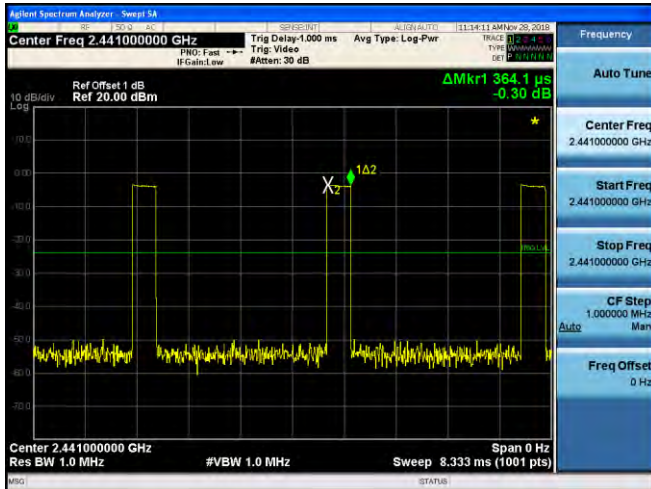
Middle Channel / 2441 MHz - DH1
