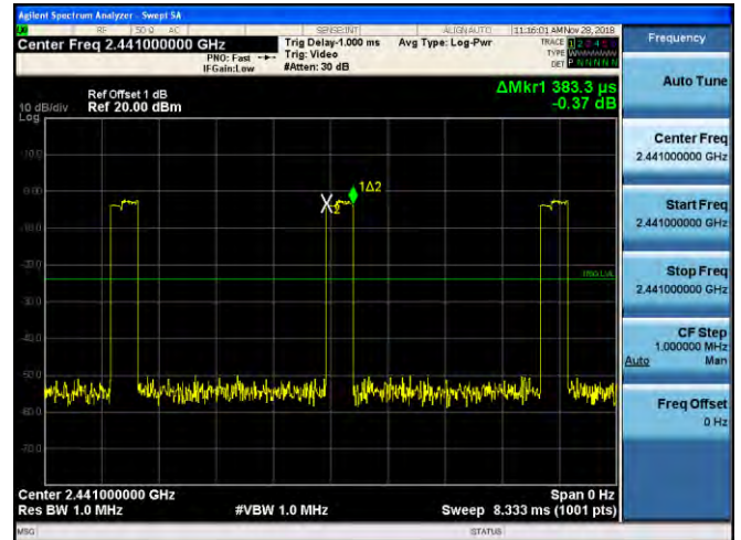
Middle Channel / 2441 MHz - 2DH1
