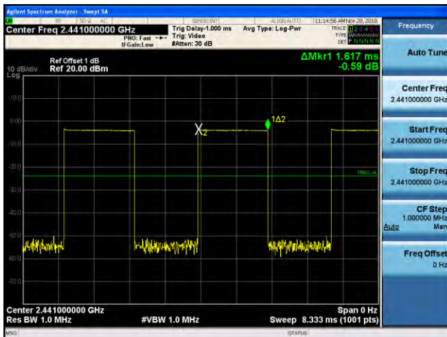
Middle Channel / 2441 MHz - DH3
