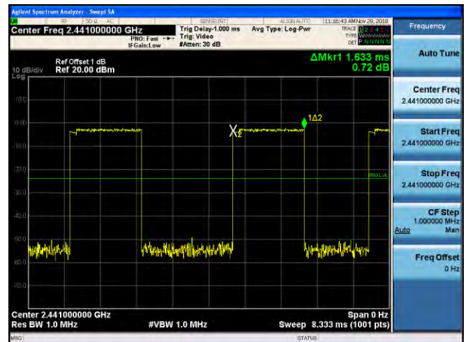
Middle Channel / 2441 MHz - 2DH3
