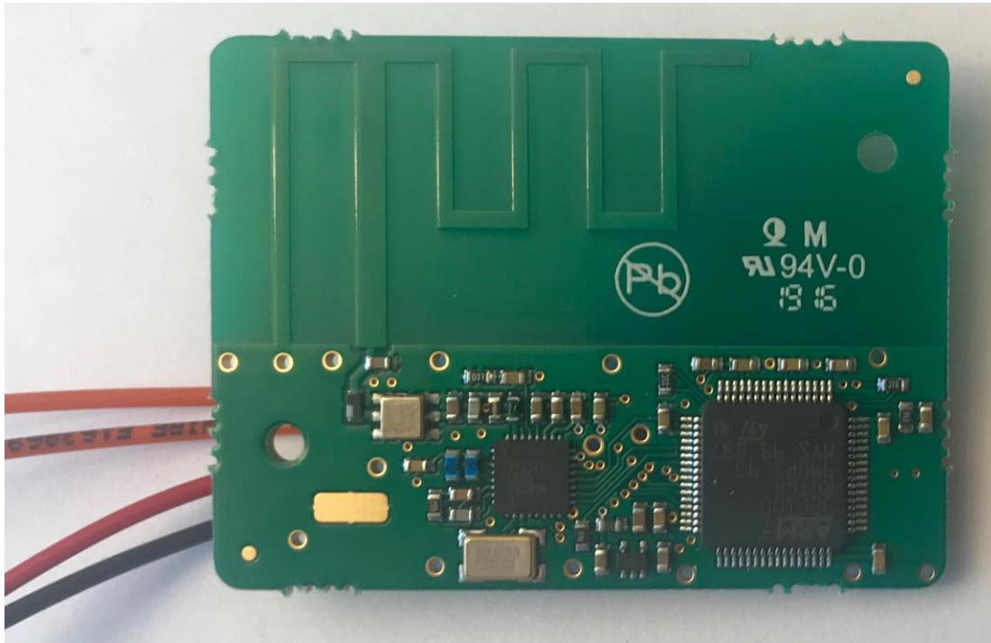
EPM-1000 pcb (molded into the top lid), front.
