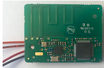
Top side.
