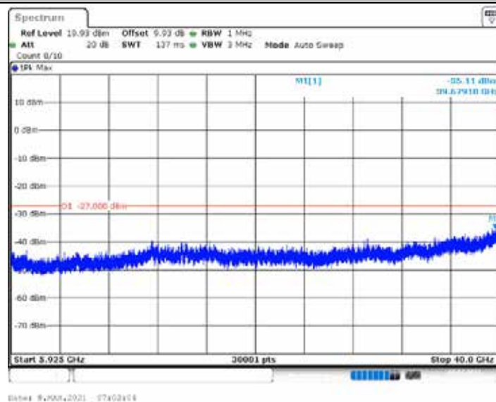
11AC20SISO_Ant1_5745_5925~40000
