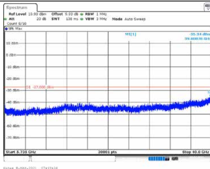
11AX20SISO_Ant1_5700_5735~40000
