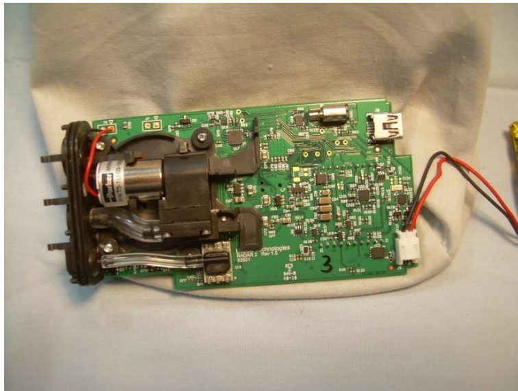
Photograph 2 – Top View of the PCB
