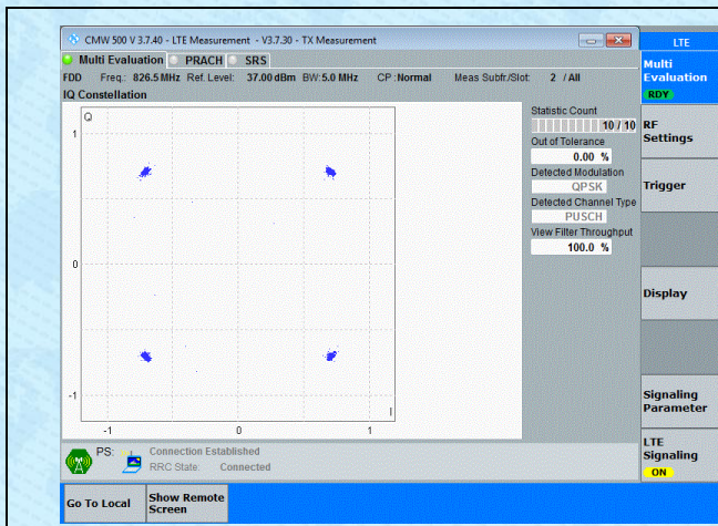
Band5-5MHz-QPSK-20425-25RB#0-PASS
