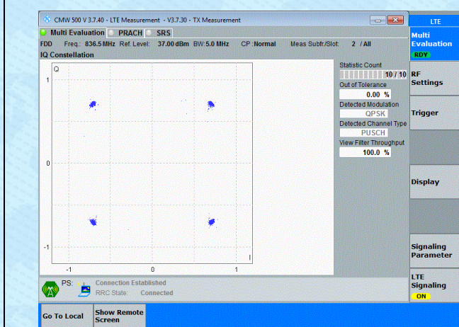
Band5-5MHz-QPSK-20525-25RB#0-PASS
