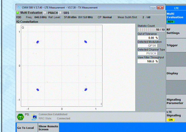
Band5-5MHz-QPSK-20625-25RB#0-PASS
