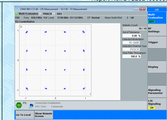
Band5-5MHz-16QAM-20425-25RB#0-PASS
