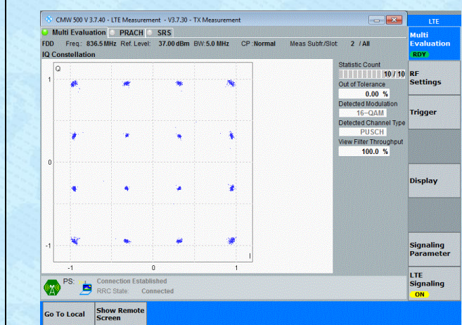
Band5-5MHz-16QAM-20525-25RB#0-PASS
