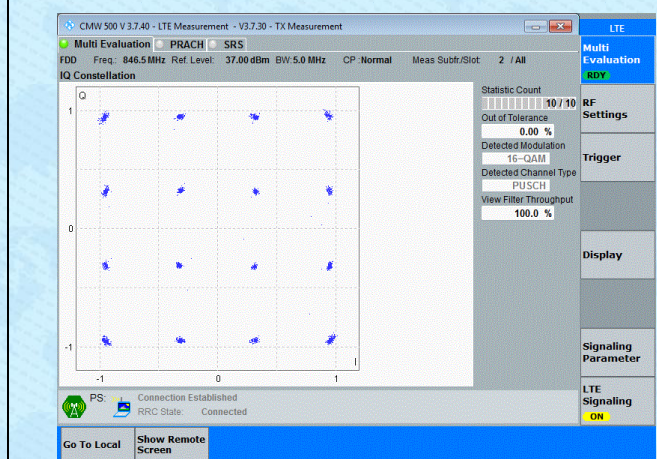
Band5-5MHz-16QAM-20625-25RB#0-PASS
