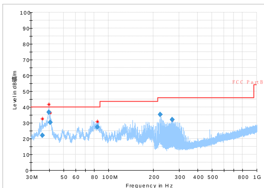
Fig 64. Radiated Spurious Emission (802.11g, Ch1, 30MHz~1GHz)
