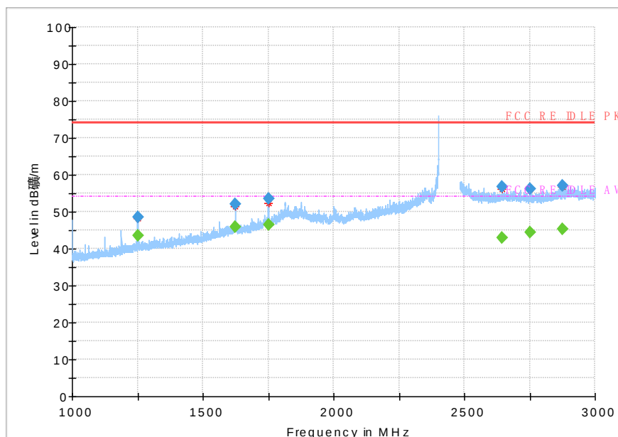
Fig 65. Radiated Spurious Emission (802.11g,Ch1,1GHz~3GHz)
