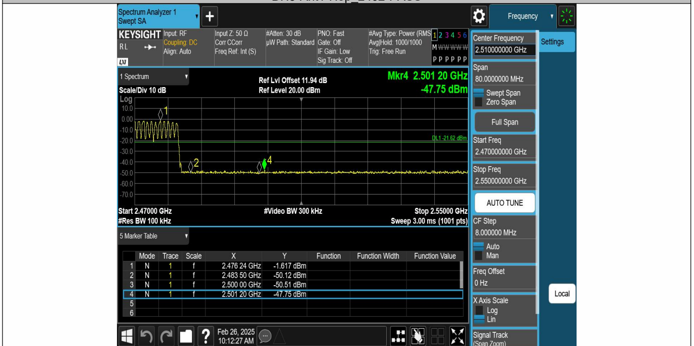
DH5-Ant1-Hop_2480-PASS
