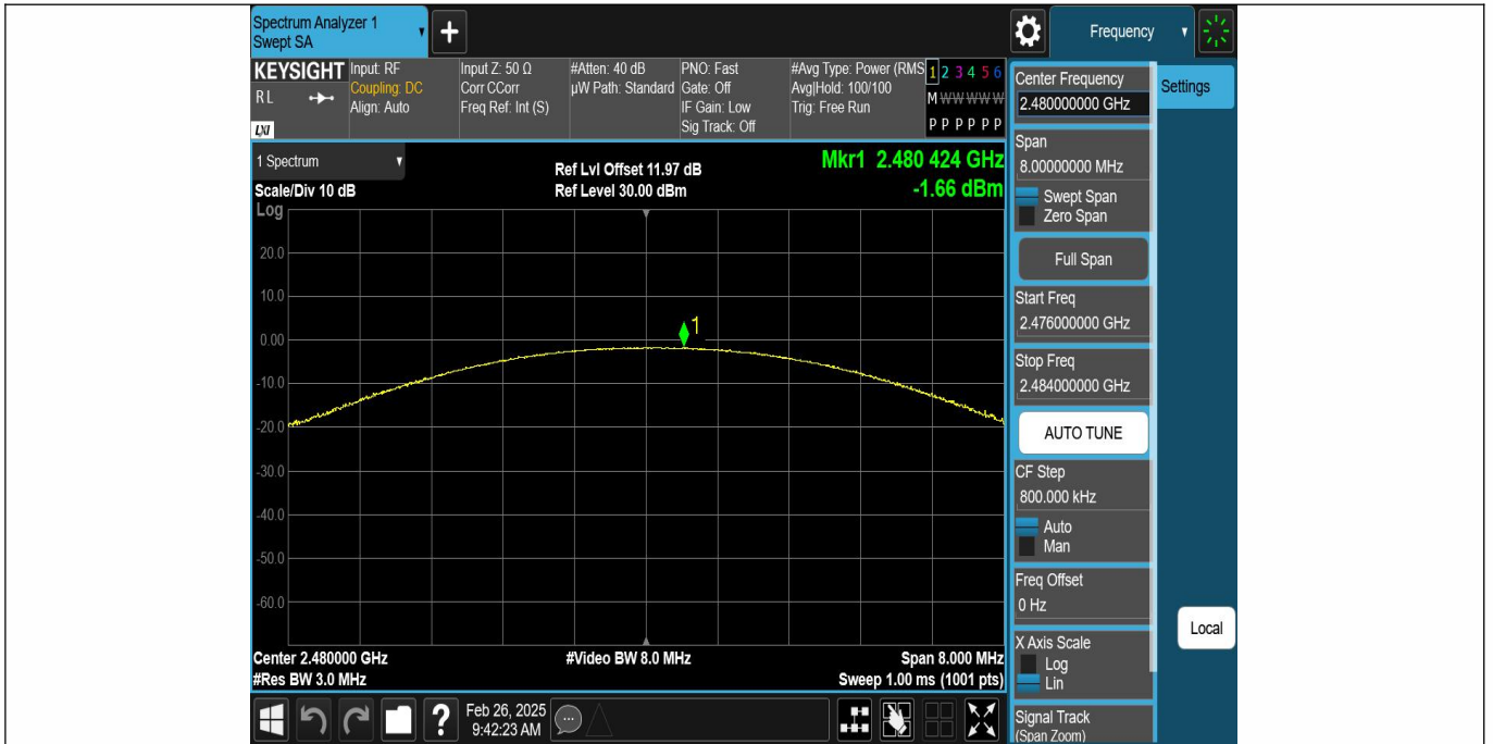
DH5-Ant1-2480-PASS
