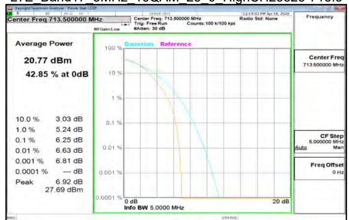
LTE Band17 5MHz 16QAM 25 0 HighCH23825-713.5
