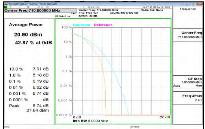
LTE Band17 5MHz 16QAM 25 0 MidCH23790-710
