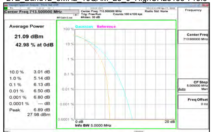
LTE Band12 5MHz 16QAM 25 0 HighCH23155-713.5
