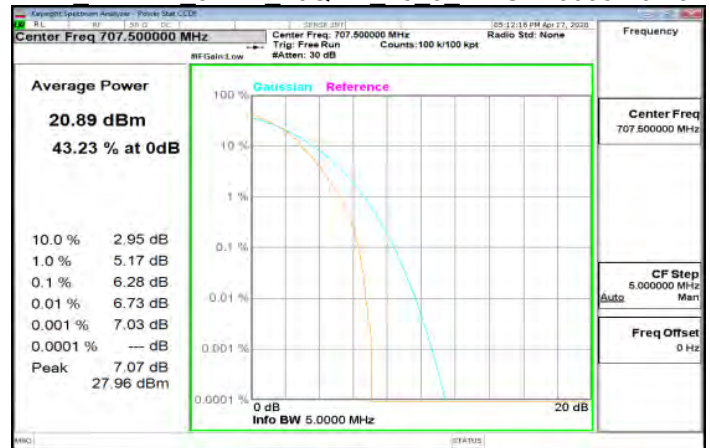
LTE Band12 5MHz 16QAM 25 0 MidCH23095-707.5
