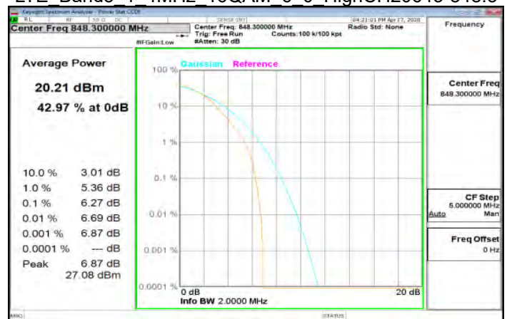
LTE Band5 1 4MHz 16QAM 6 0 HighCH20643-848.3
