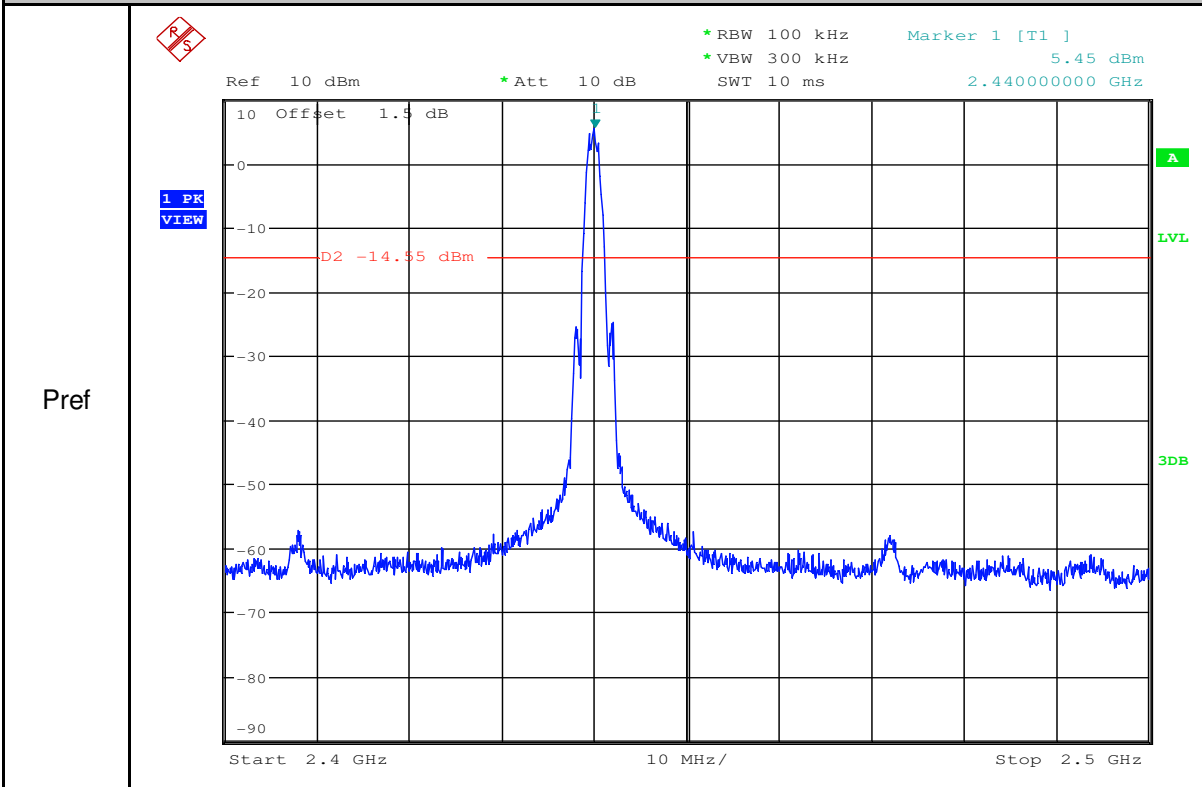
RF Conducted Spurious Emissions_BLE_2440_Ant1_2Mbps
