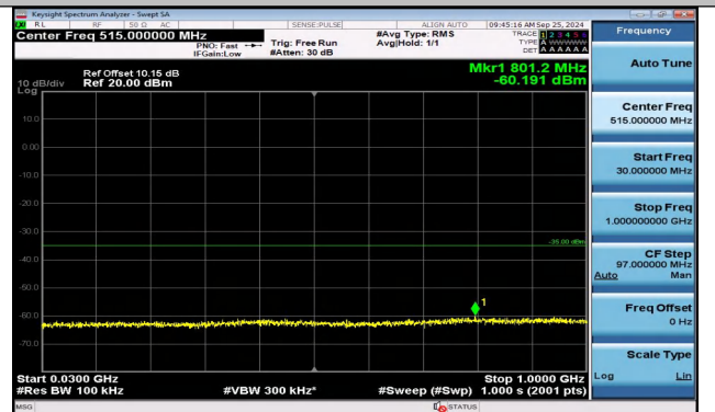
Band38_5MHz_16QAM_38000_25RB#0_30~1000_30~10 00
