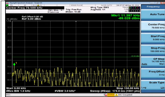
Band38_5MHz_QPSK_37775_1RB#24_0.009~0.15_0.009 ~0.15
