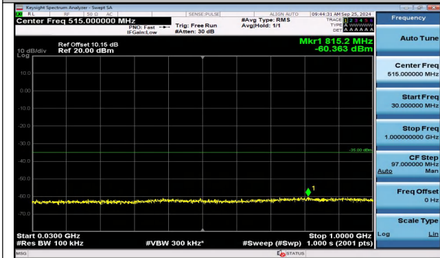
Band38_5MHz_QPSK_38000_25RB#0_30~1000_30~100 0
