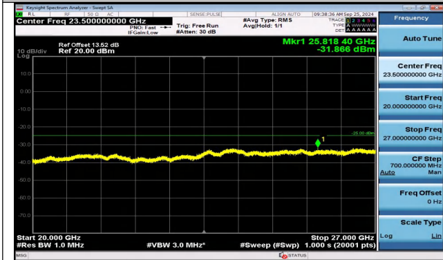
Band38_5MHz_QPSK_37775_1RB#24_20000~27000_20 000~27000
