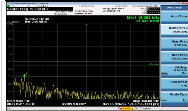
Band38_5MHz_QPSK_38000_25RB#0_0.009~0.15_0.009 ~0.15
