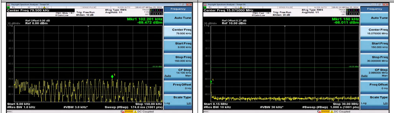
Band38_5MHz_QPSK_38000_1RB#0_0.009~0.15_0.009~
