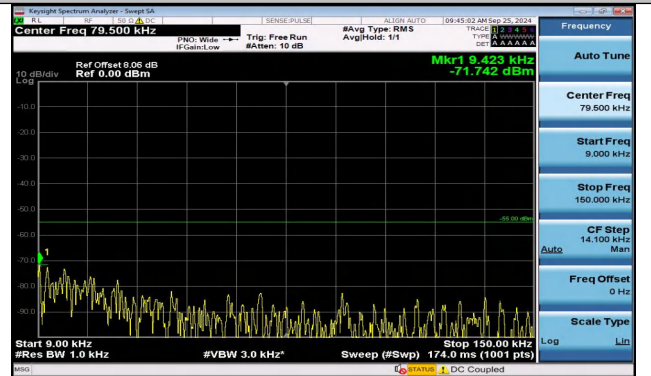
Band38_5MHz_16QAM_38000_25RB#0_0.009~0.15_0.00 9~0.15
