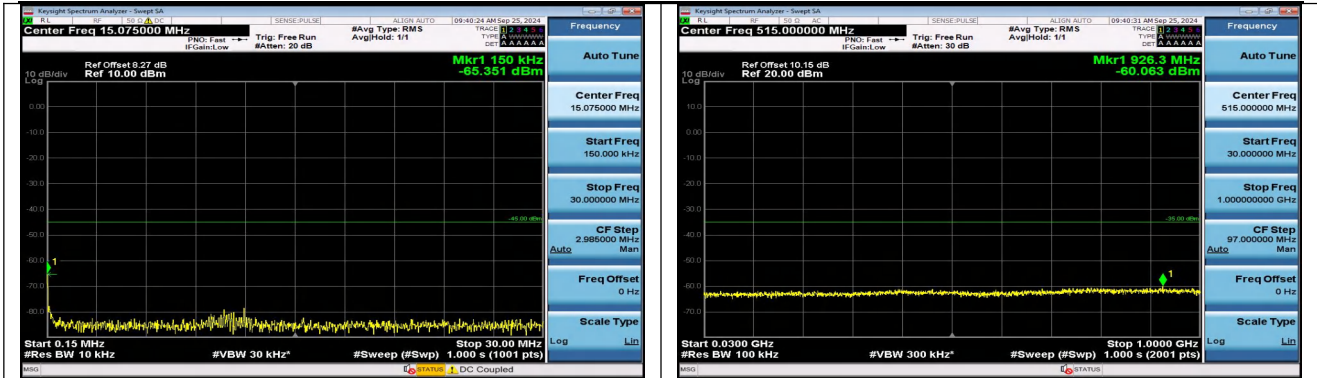
Band38_5MHz_16QAM_37775_25RB#0_0.15~30_0.15~3
