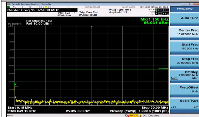
Band38_5MHz_16QAM_38000_25RB#0_0.15~30_0.15~3 0
