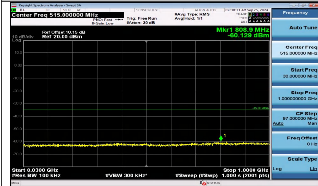
Band38_5MHz_QPSK_37775_1RB#24_30~1000_30~100 0
