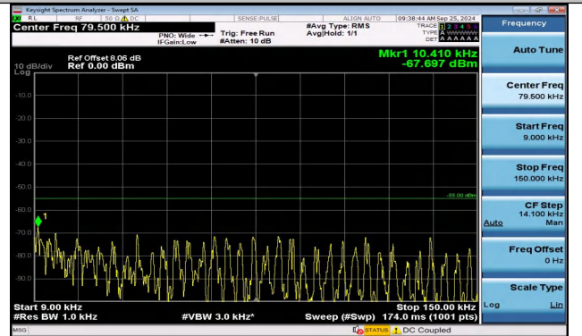
Band38_5MHz_16QAM_37775_1RB#24_0.009~0.15_0.00 9~0.15
