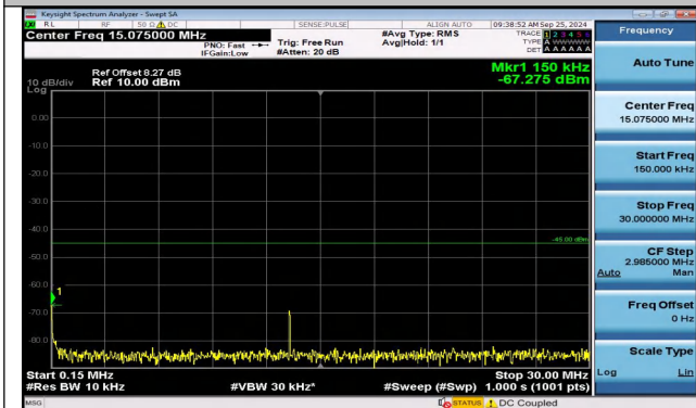
Band38_5MHz_16QAM_37775_1RB#24_0.15~30_0.15~3 0
