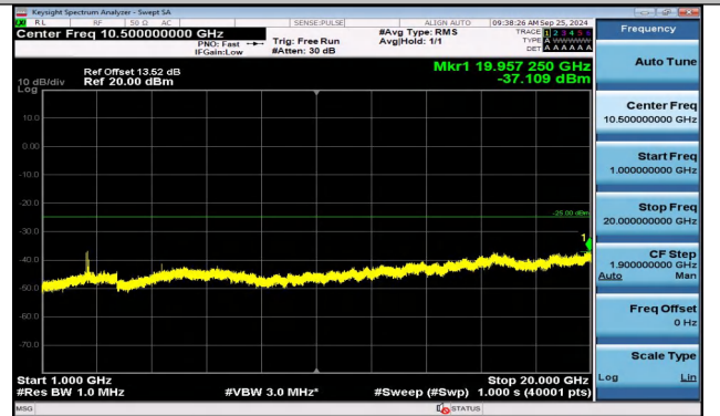
Band38_5MHz_QPSK_37775_1RB#24_1000~20000_100 0~20000
