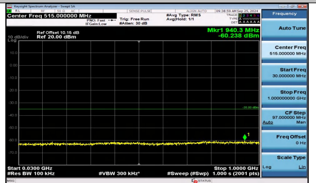
Band38_5MHz_16QAM_37775_1RB#24_30~1000_30~10 00
