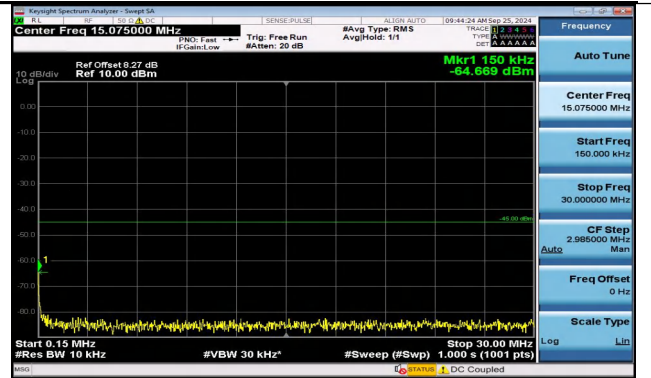
Band38_5MHz_QPSK_38000_25RB#0_0.15~30_0.15~30
