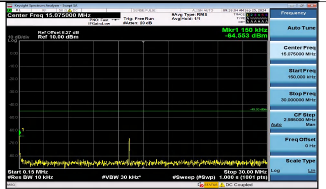
Band38_5MHz_QPSK_37775_1RB#24_0.15~30_0.15~30
