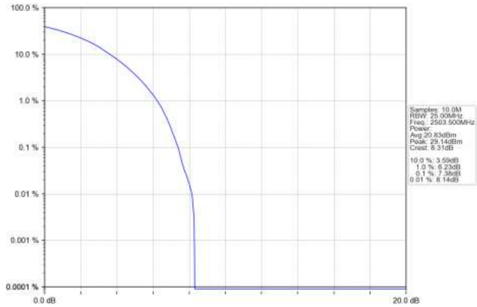
n41_30kHz_SISO_NTNV_15MHz_CP-OFDM_QPSK_2503.5MHz_Outer_Full_Ant1
