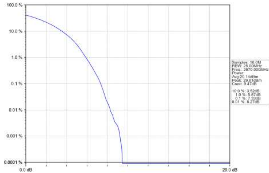
n41_30kHz_SISO_NTNV_40MHz_DFT-s-OFDM_64_QAM_2670MHz_Outer_Full_Ant1
