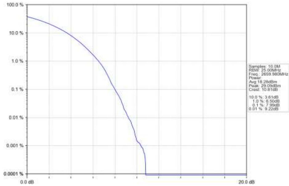
n41_30kHz_SISO_NTNV_60MHz_CP-OFDM_QPSK_2659.98MHz_Outer_Full_Ant1
