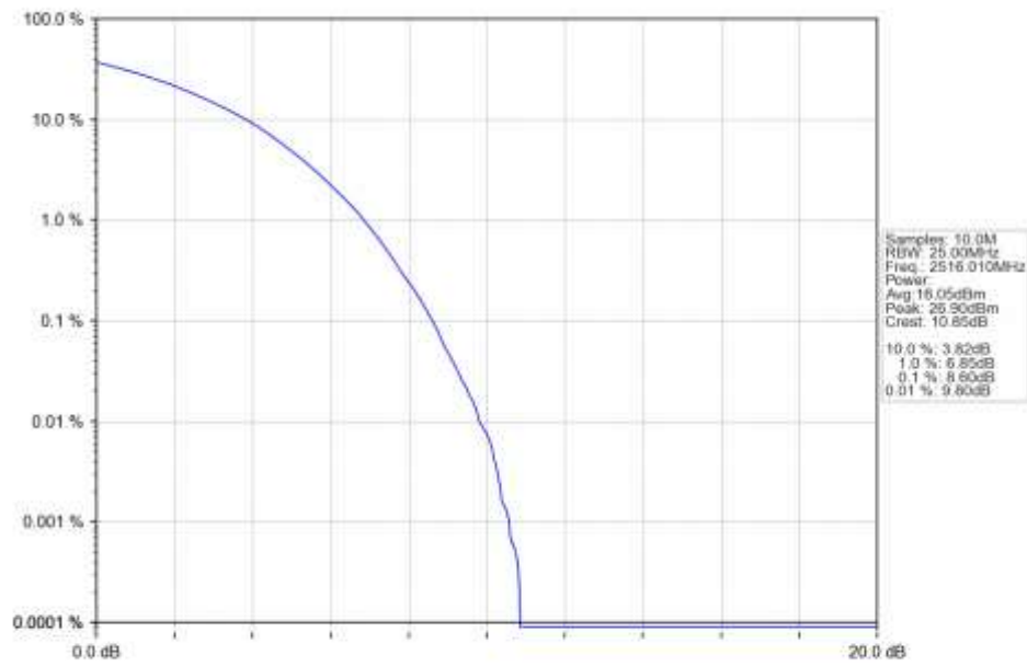
n41_30kHz_SISO_NTNV_40MHz_CP-OFDM_256_QAM_2516.01MHz_Outer_Full_Ant1
