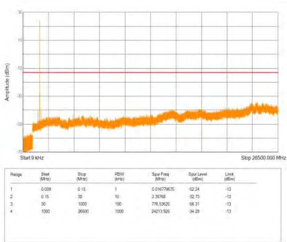
Band4 QPSK BW=5MHz Channel=20175 RB Size=6 Position=#0 NB Index=0
