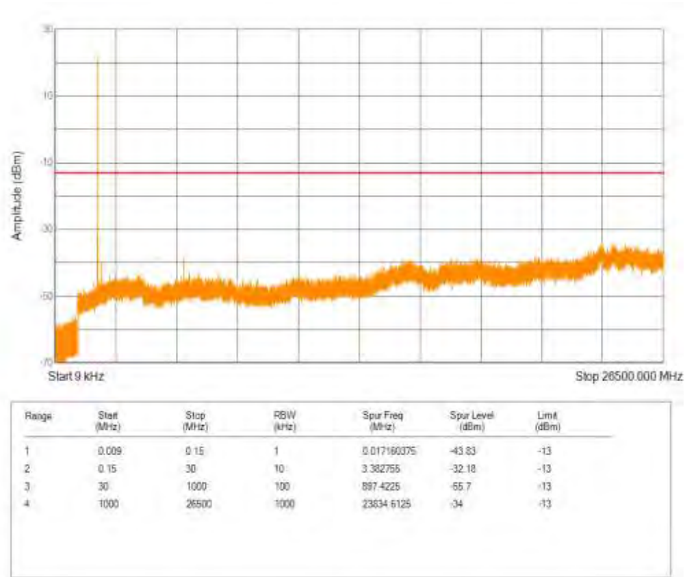
Band25 QPSK BW=20MHz Channel=26365 RB Size=6 Position=#0 NB Index=0
