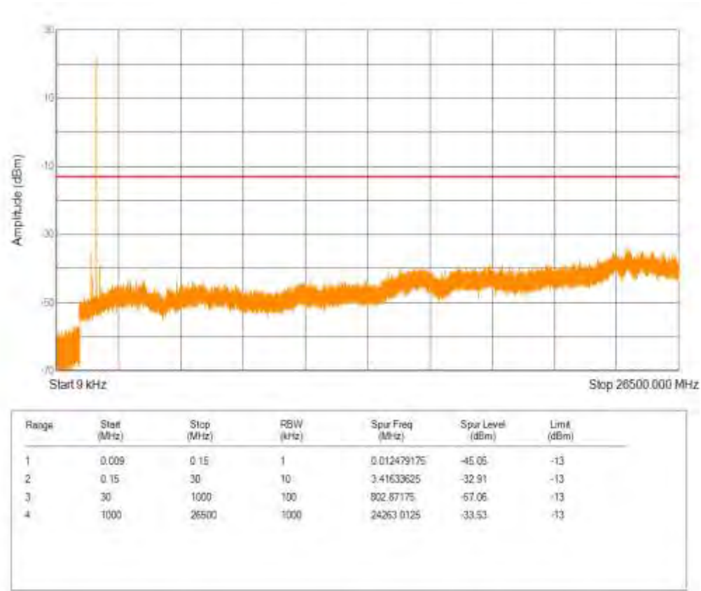
Band66 16QAM BW=10MHz Channel=132022 RB Size=1 Position=#0 NB Index=0
