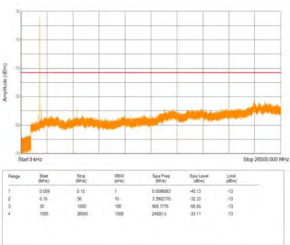
Band25 16QAM BW=10MHz Channel=26640 RB Size=5 Position=#0 NB Index=0
