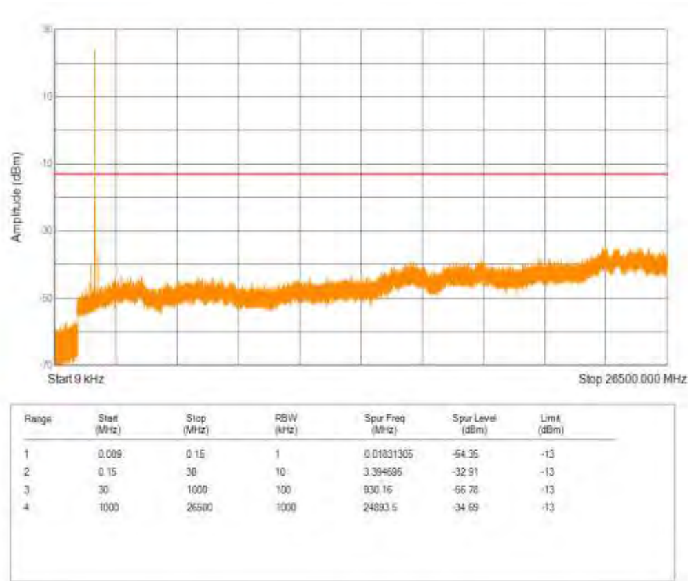
Band4 16QAM BW=20MHz Channel=20300 RB Size=5 Position=#0 NB Index=0
