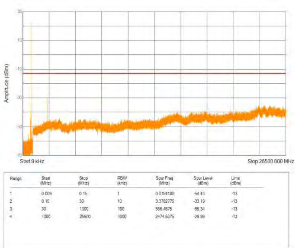
Band5 QPSK BW=10MHz Channel=20450 RB Size=6 Position=#0 NB Index=0
