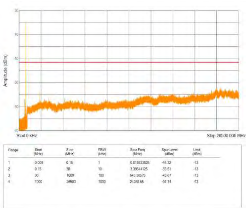
Band26(824-849) QPSK BW=1.4MHz Channel=26915 RB Size=6 Position=#0 NB Index=0
