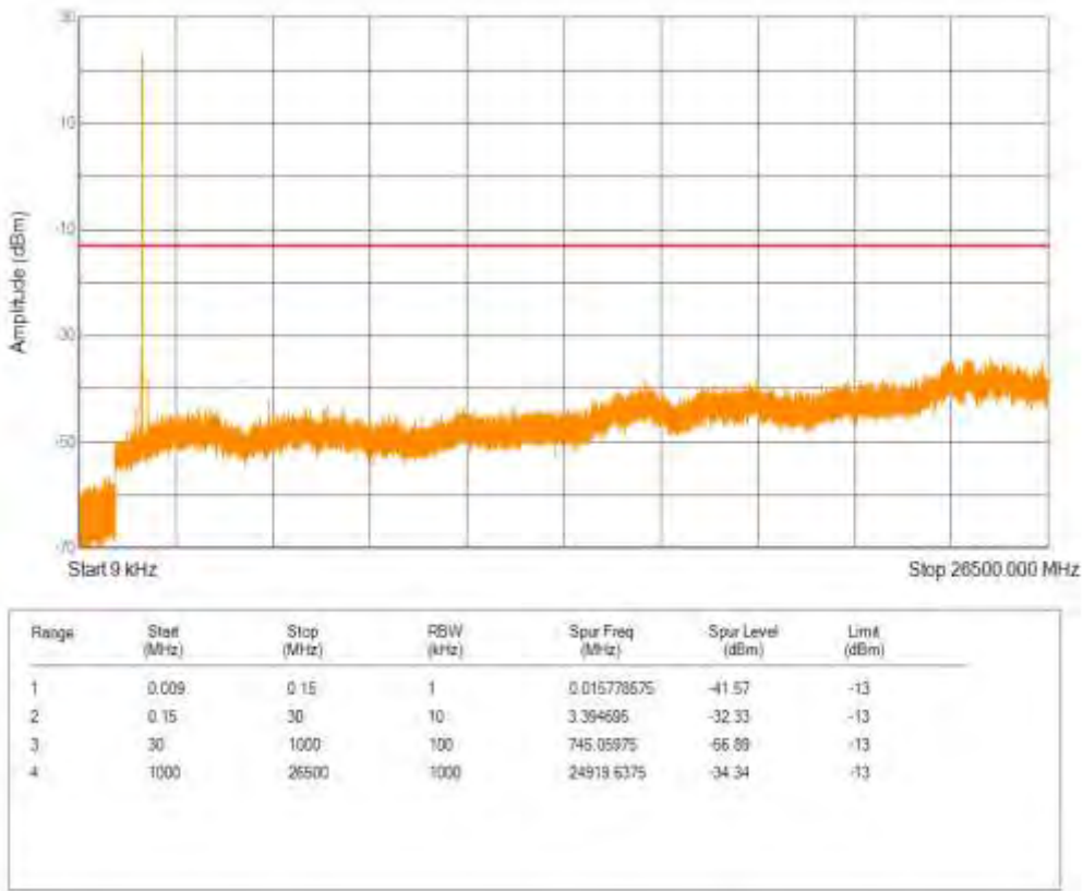
Band66 16QAM BW=15MHz Channel=132322 RB Size=1 Position=#0 NB Index=0
