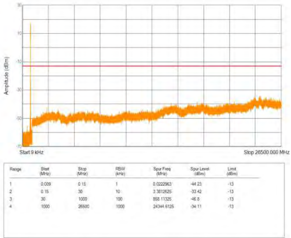
Band26(824-849) 16QAM BW=1.4MHz Channel=26915 RB Size=1 Position=#0 NB Index=0
