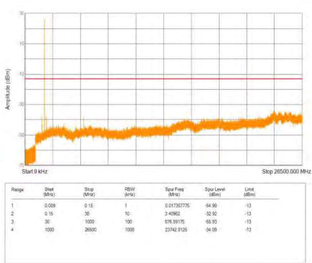
Band2 QPSK BW=10MHz Channel=18900 RB Size=6 Position=#0 NB Index=0
