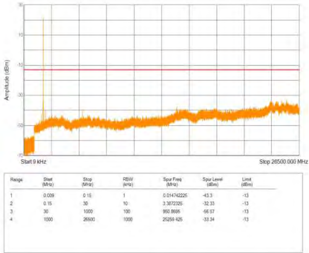
Band25 16QAM BW=15MHz Channel=26365 RB Size=1 Position=#0 NB Index=0
