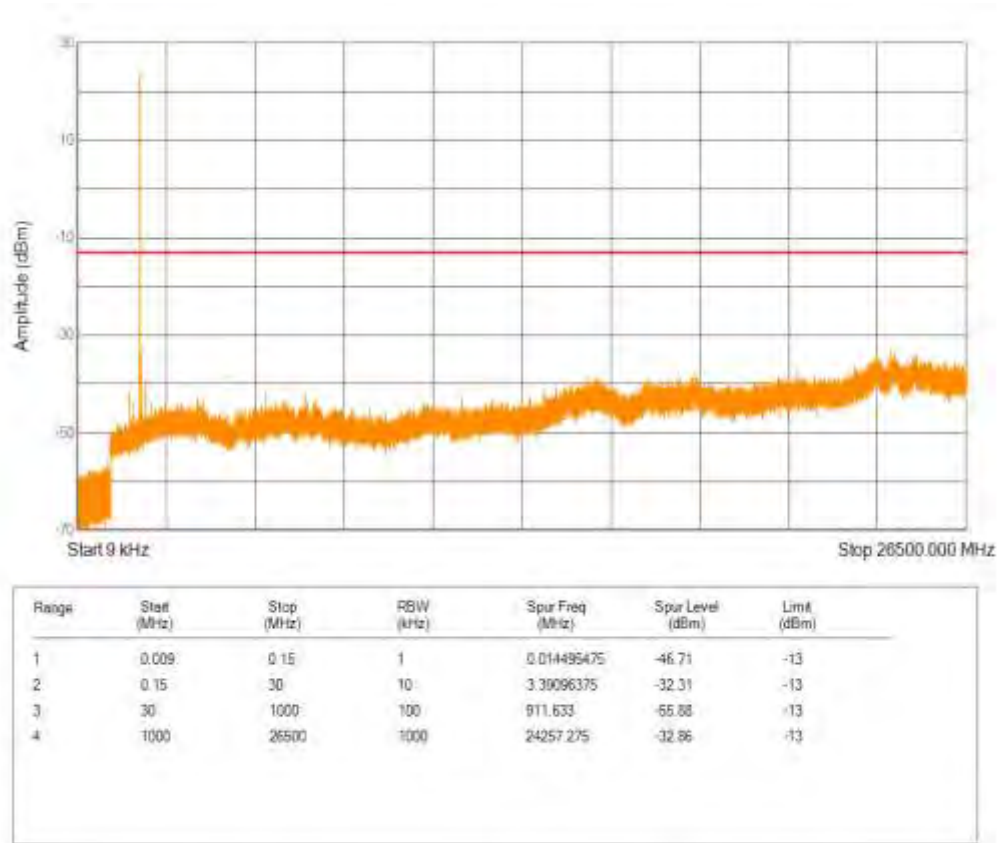
Band25 QPSK BW=15MHz Channel=26365 RB Size=6 Position=#0 NB Index=0
