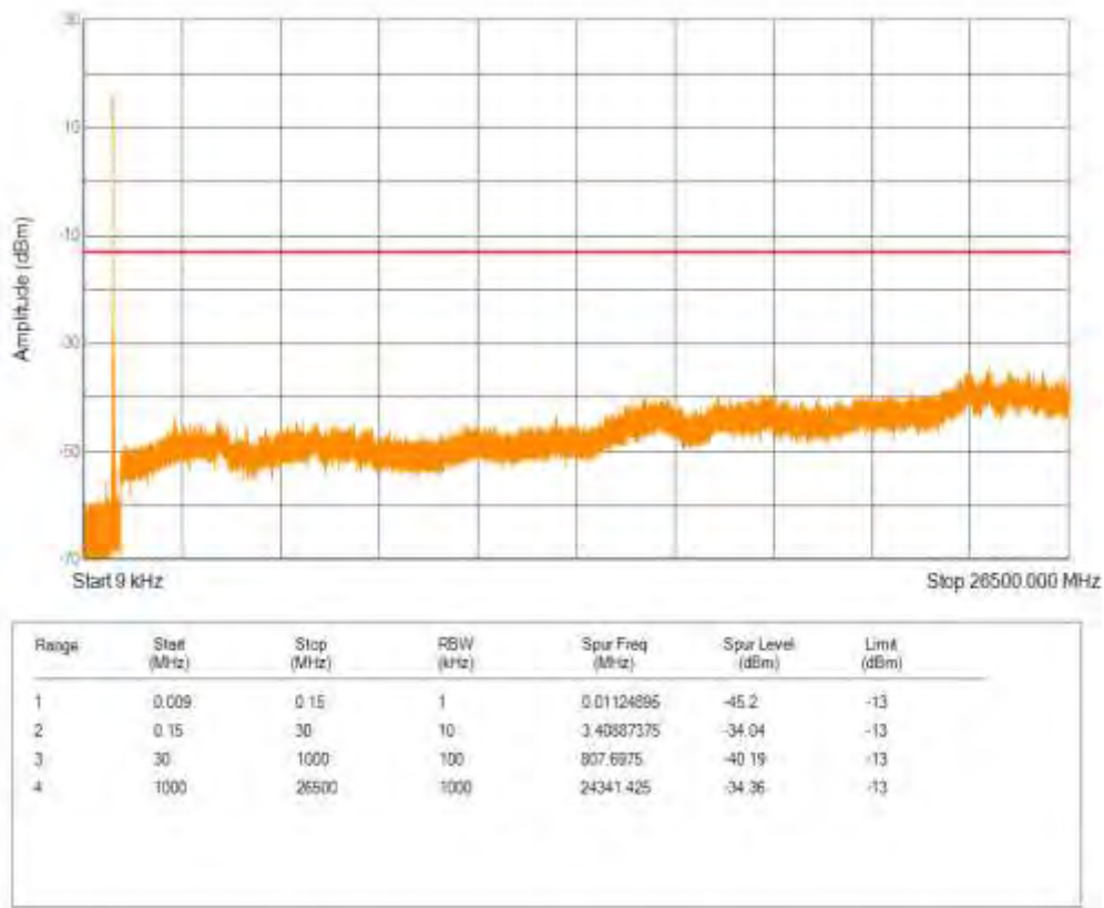
Band26(814-824) 16QAM BW=1.4MHz Channel=26740 RB Size=1 Position=#0 NB Index=0
