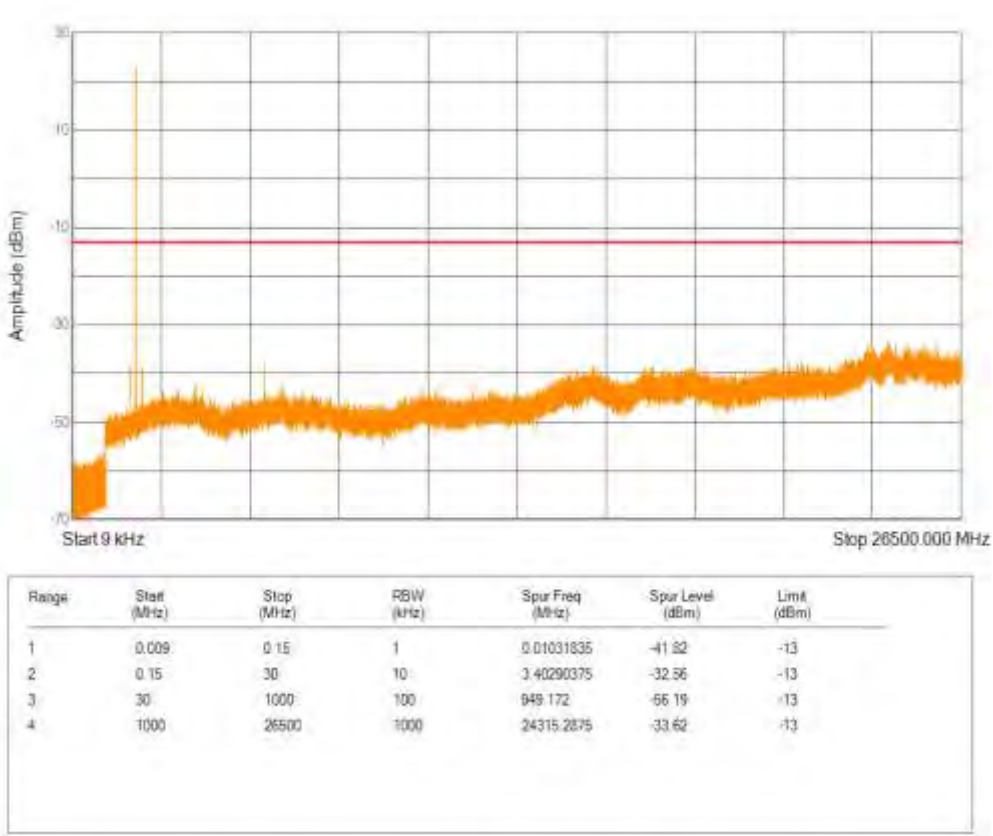
Band25 QPSK BW=15MHz Channel=26115 RB Size=1 Position=#0 NB Index=0
