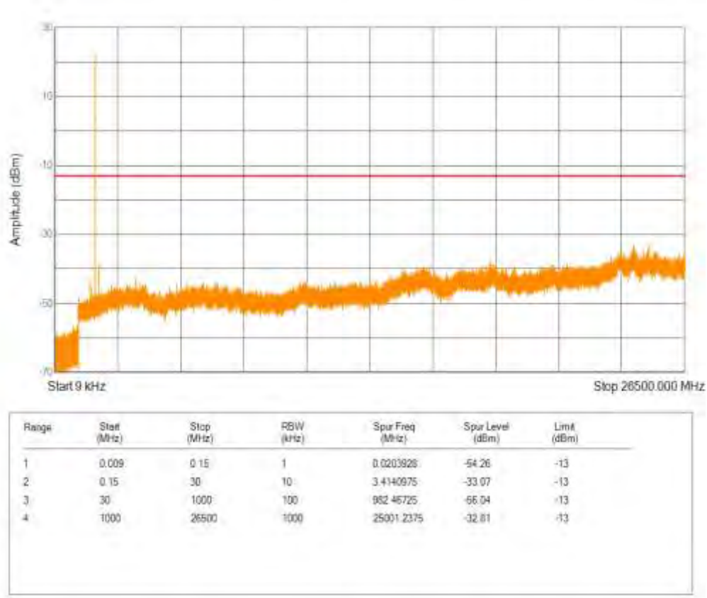
Band4 16QAM BW=3MHz Channel=19965 RB Size=1 Position=#0 NB Index=0
