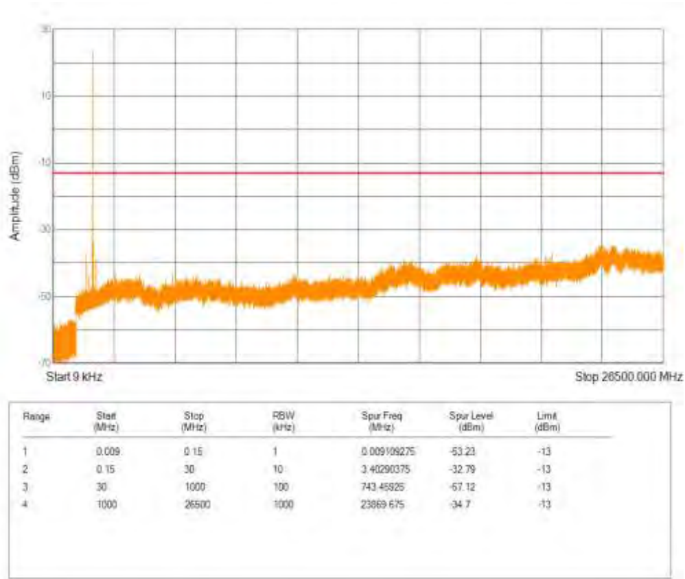
Band4 16QAM BW=10MHz Channel=20175 RB Size=1 Position=#0 NB Index=0
