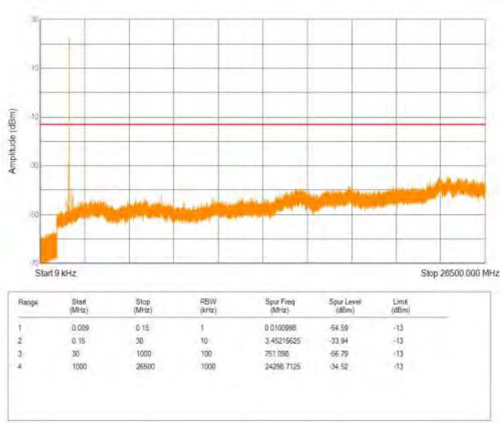
Band4 16QAM BW=5MHz Channel=20175 RB Size=1 Position=#0 NB Index=0
