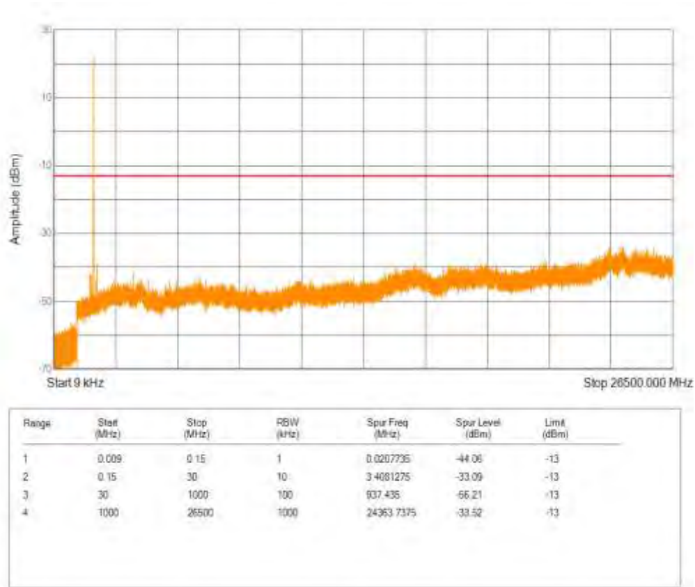
Band66 QPSK BW=3MHz Channel=131987 RB Size=6 Position=#0 NB Index=0
