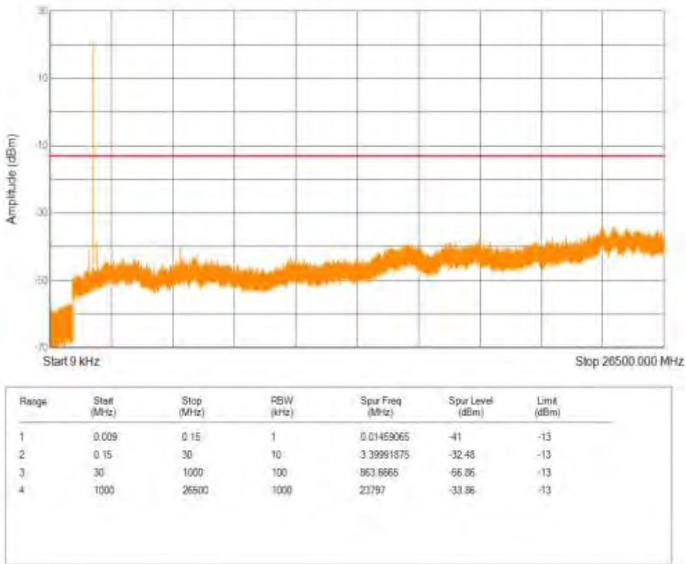
Band25 16QAM BW=10MHz Channel=26365 RB Size=5 Position=#0 NB Index=0
