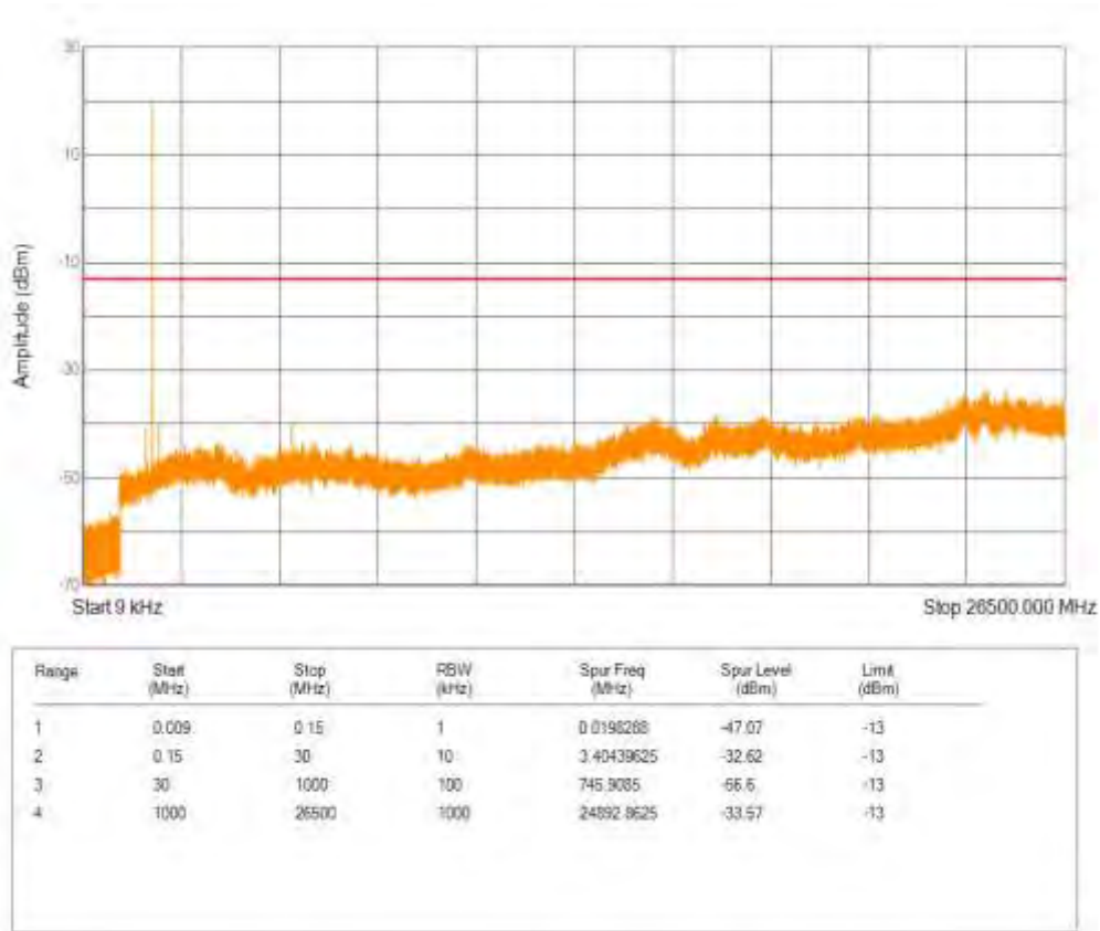
Band25 16QAM BW=5MHz Channel=26365 RB Size=5 Position=#0 NB Index=0
