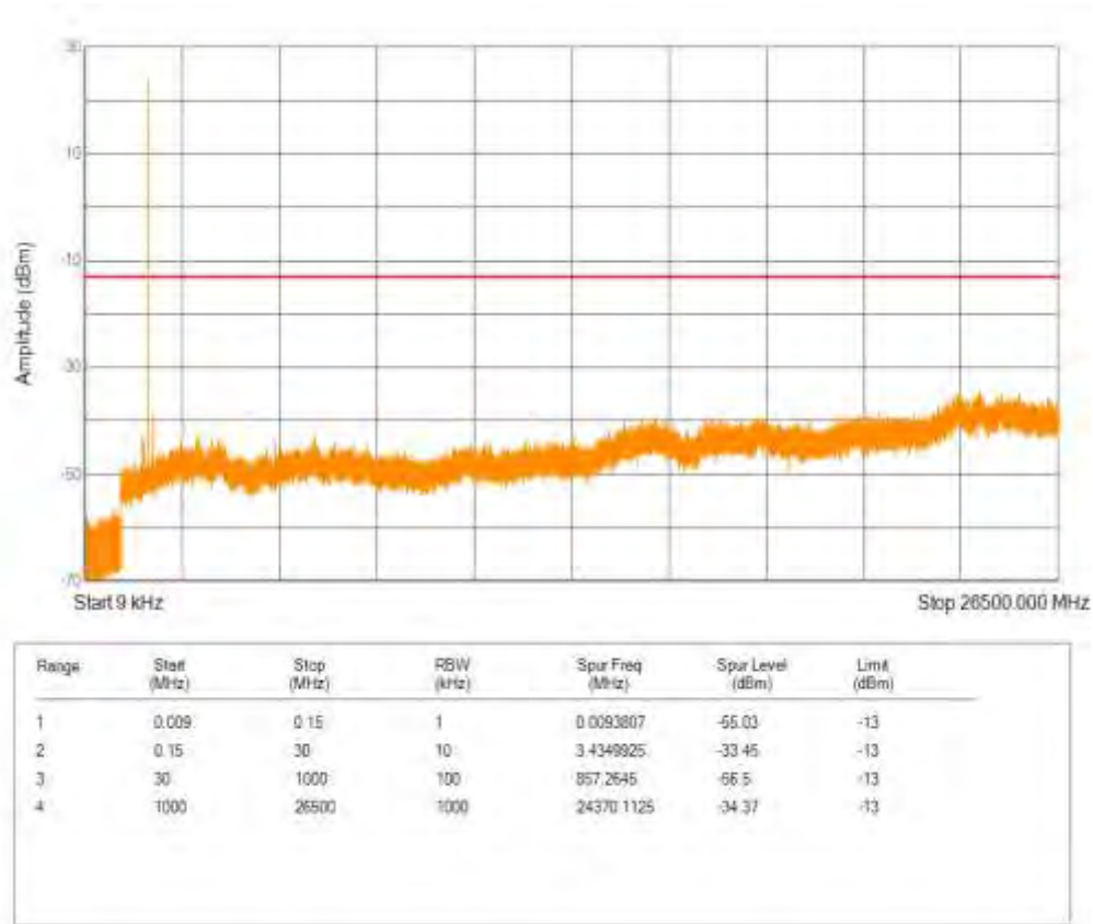
Band4 QPSK BW=10MHz Channel=20175 RB Size=6 Position=#0 NB Index=0
