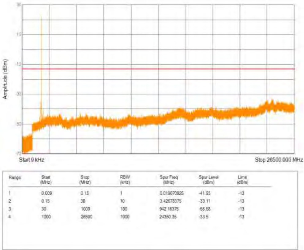
Band25 16QAM BW=3MHz Channel=26365 RB Size=1 Position=#0 NB Index=0
