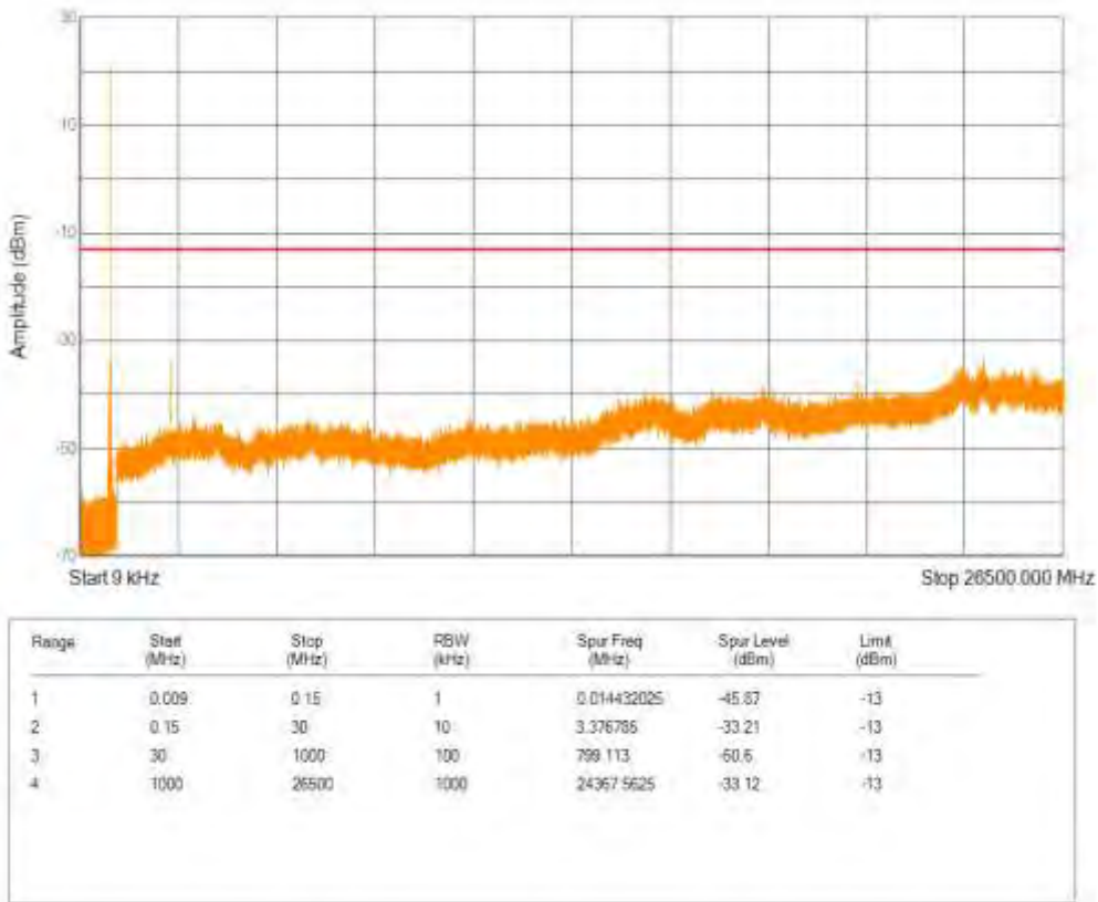
Band26(824-849) QPSK BW=3MHz Channel=26805 RB Size=6 Position=#0 NB Index=0
