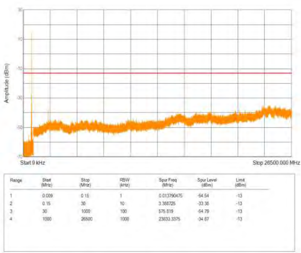
Band5 16QAM BW=10MHz Channel=20450 RB Size=1 Position=#0 NB Index=0
