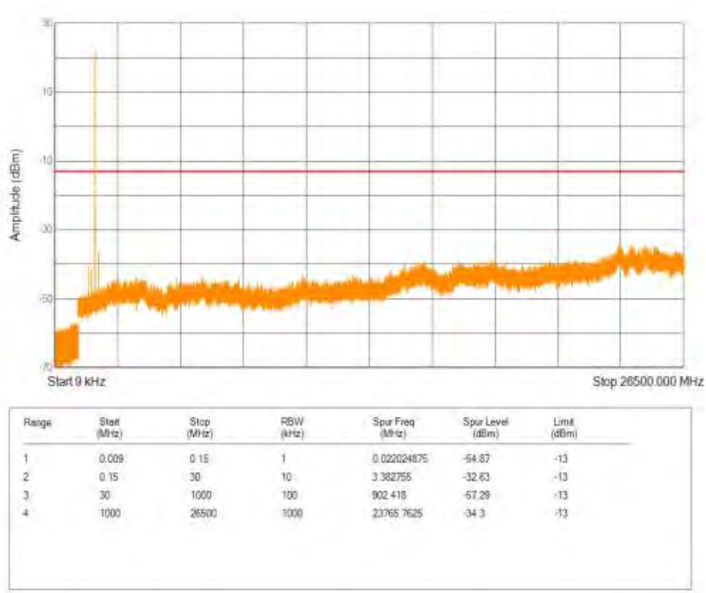
Band4 QPSK BW=1.4MHz Channel=20175 RB Size=1 Position=#0 NB Index=0
