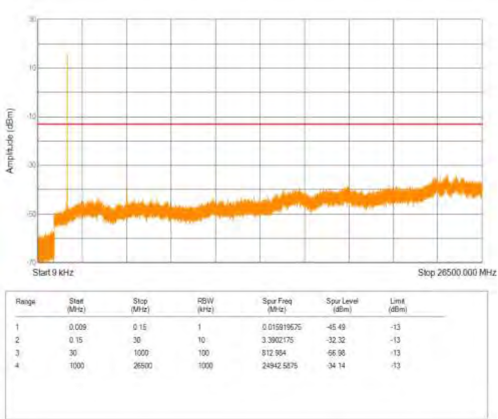
Band66 16QAM BW=3MHz Channel=132657 RB Size=5 Position=#0 NB Index=0
