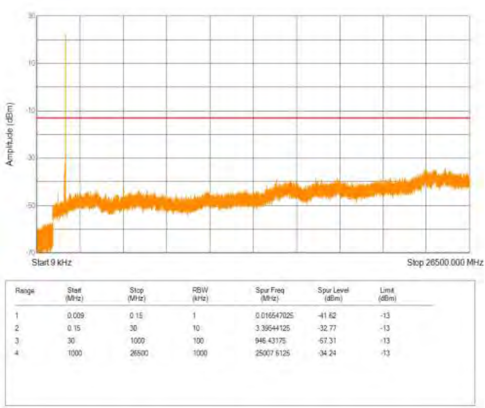
Band66 QPSK BW=5MHz Channel=131997 RB Size=1 Position=#0 NB Index=0
