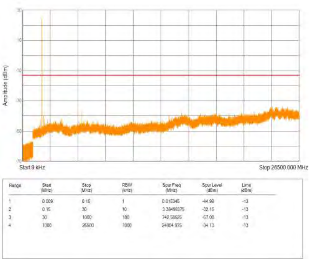
Band25 QPSK BW=15MHz Channel=26615 RB Size=1 Position=#0 NB Index=0
