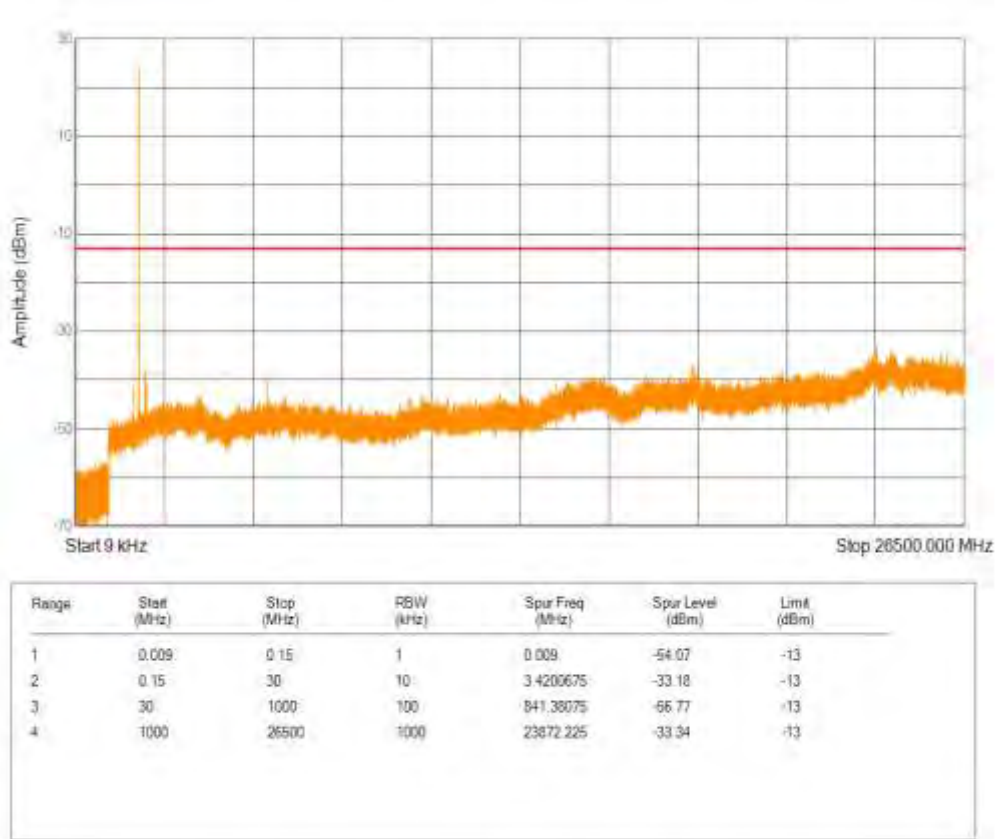
Band2 16QAM BW=3MHz Channel=19185 RB Size=5 Position=#0 NB Index=0
