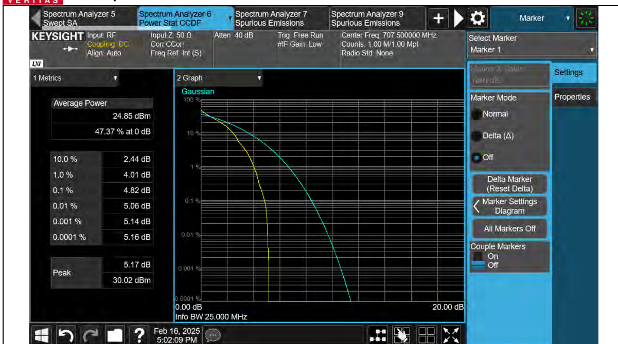
Band12-10MHz-QPSK-23095-50RB#0
