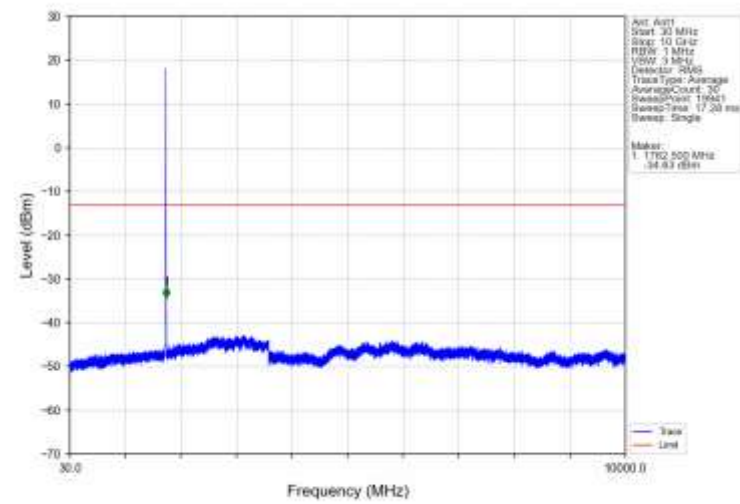
Band4_RMC_HCH_1752.6MHz_12.2kbps_RMC_NTNV
