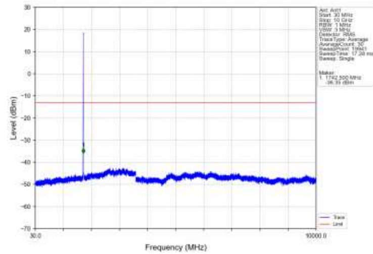
Band4_RMC_MCH_1732.6MHz_12.2kbps_RMC_NTNV
