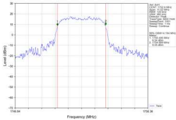
Band4_HSDPA_HCH_1752.6MHz_Subtest 1_NTNV
