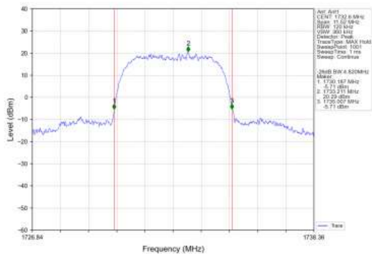
Band4_RMC_MCH_1732.6MHz_12.2kbps RMC_NTNV
