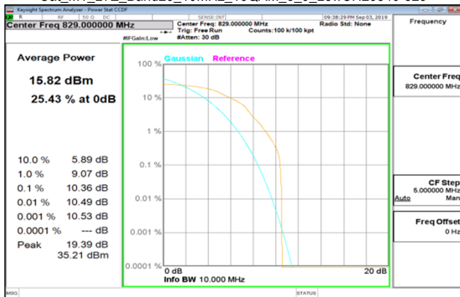
Cat_M1_LTE_Band26_10MHz_16QAM_6_0_LowCH26840-829
