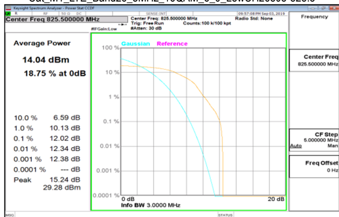
Cat M1_LTE_Band26_3MHz_16QAM_6_0_LowCH26805-825.5
