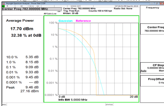
Cat_M1_LTE_Band13_5MHz_16QAM_6_0_MidCH23230-782
