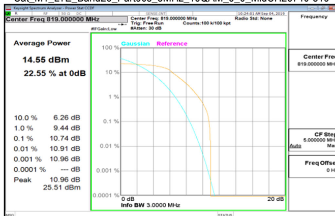
Cat M1 LTE_Band26_Part90s_3MHz_16QAM_6_0_MidCH26740-819
