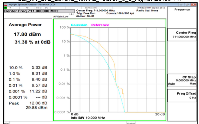
Cat_M1_LTE_Band12_10MHz_16QAM_6_0_HighCH23130-711
