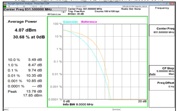
Cat_M1_LTE_Band26_15MHz_16QAM_6_0_LowCH26865-831.5
