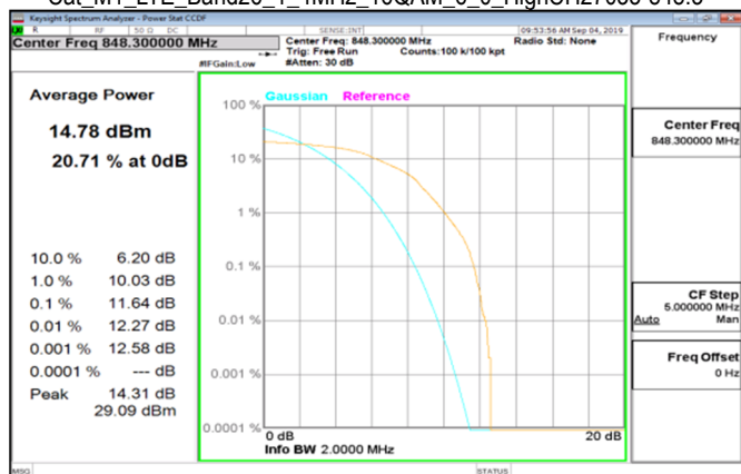
Cat M1_LTE_Band26_1_4MHz_16QAM_6_0_HighCH27033-848.3
