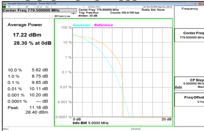
Cat_M1_LTE_Band13_5MHz_16QAM_6_0_LowCH23205-779.5
