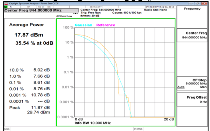
Cat_M1_LTE_Band26_10MHz_16QAM_6_0_HighCH26990-844
