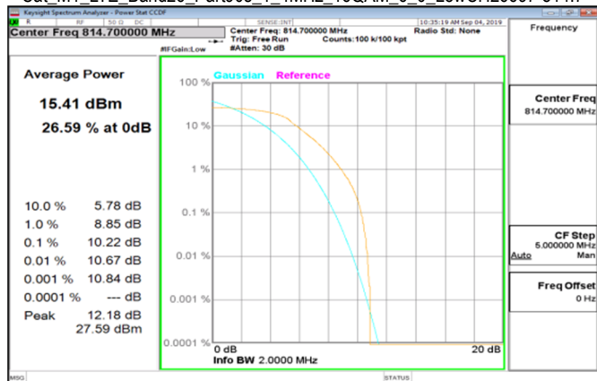
Cat M1 LTE_Band26_Part90s_1_4MHz_16QAM_6_0_LowCH26697-814.7
