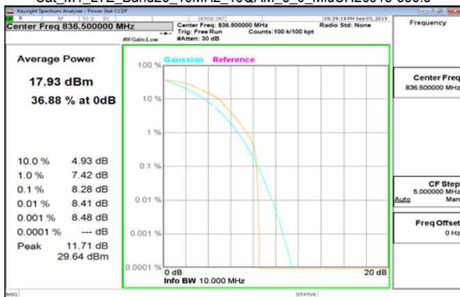
Cat_M1_LTE_Band26_10MHz_16QAM_6_0_MidCH26915-836.5
