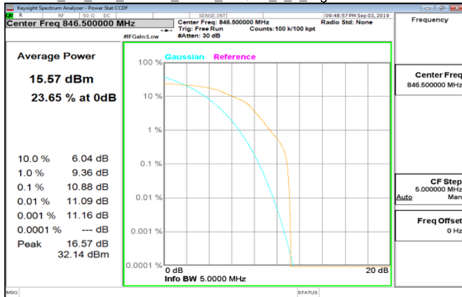
Cat_M1_LTE_Band26_5MHz_16QAM_6_0_HighCH27015-846.5
