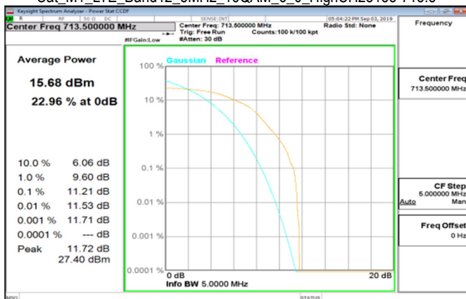
Cat_M1_LTE_Band12_5MHz_16QAM_6_0_HighCH23155-713.5
