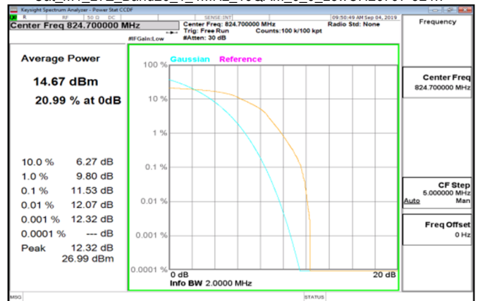
Cat_M1_LTE_Band26_1_4MHz_16QAM_6_0_LowCH26797-824.7
