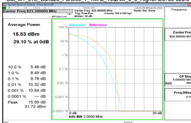
Cat M1 LTE_Band26_Part90s_1_4MHz_16QAM_6_0_HighCH26783-823.3
