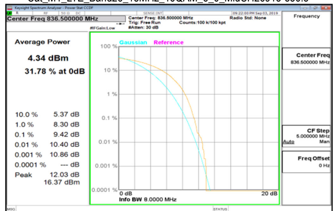
Cat_M1_LTE_Band26_15MHz_16QAM_6_0_MidCH26915-836.5
