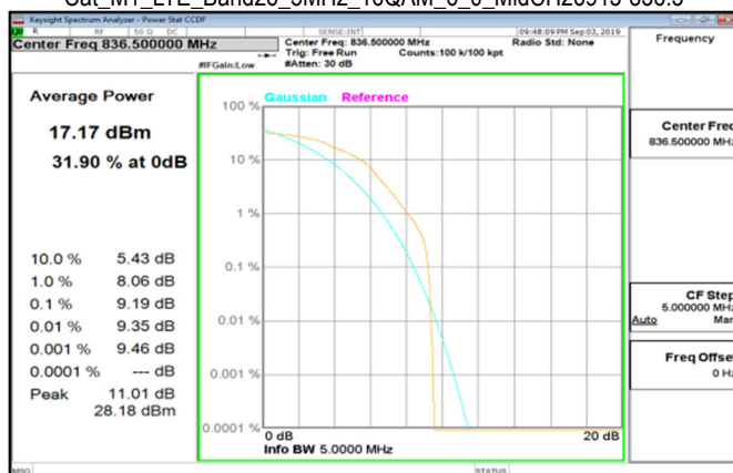
Cat M1_LTE_Band26_5MHz_16QAM_6_0_MidCH26915-836.5
