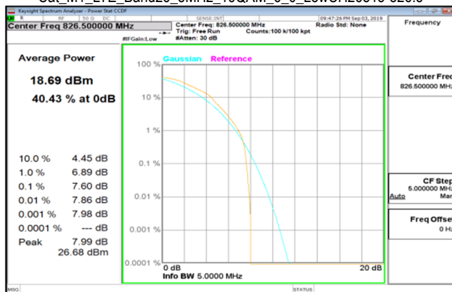
Cat M1_LTE_Band26_5MHz_16QAM_6_0_LowCH26815-826.5
