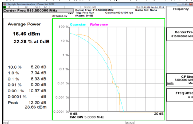
Cat M1 LTE_Band26_Part90s_3MHz_16QAM_6_0_LowCH26705-815.5
