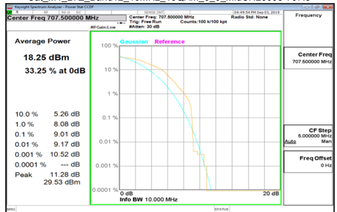
Cat_M1_LTE_Band12_10MHz_16QAM_6_0_MidCH23095-707.5
