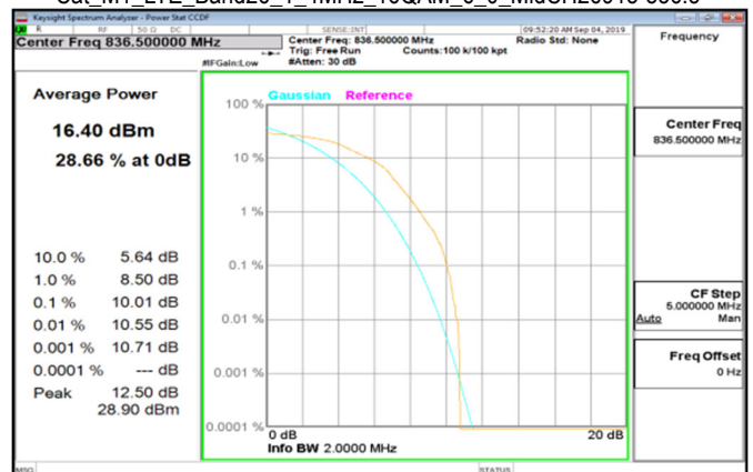
Cat_M1_LTE_Band26_1_4MHz_16QAM_6_0_MidCH26915-836.5
