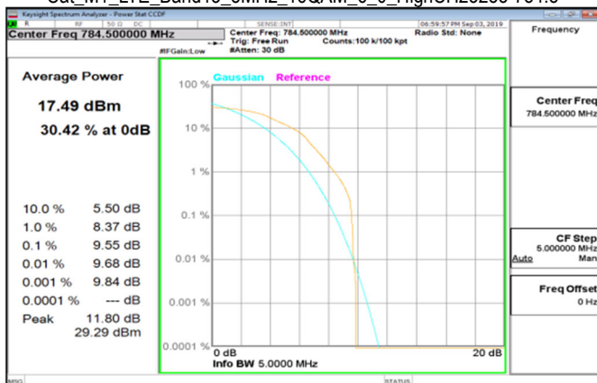
Cat_M1_LTE_Band13_5MHz_16QAM_6_0_HighCH23255-784.5
