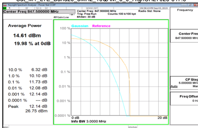
Cat M1_LTE_Band26_3MHz_16QAM_6_0_HighCH27025-847.5
