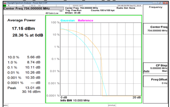
Cat_M1_LTE_Band12_10MHz_16QAM_6_0_LowCH23060-704
