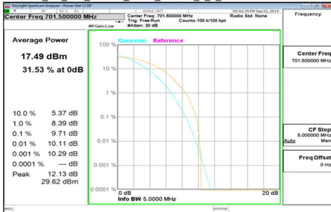
Cat_M1_LTE_Band12_5MHz_16QAM_6_0_LowCH23035-701.5
