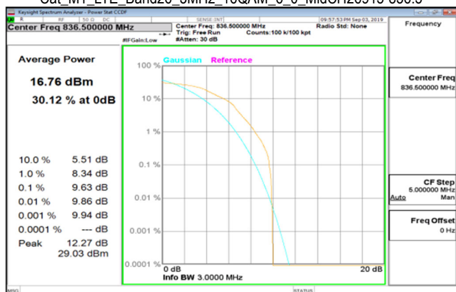
Cat M1_LTE_Band26_3MHz_16QAM_6_0_MidCH26915-836.5
