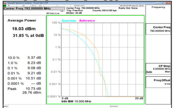
Cat_M1_LTE_Band13_10MHz_16QAM_6_0_MidCH23230-782
