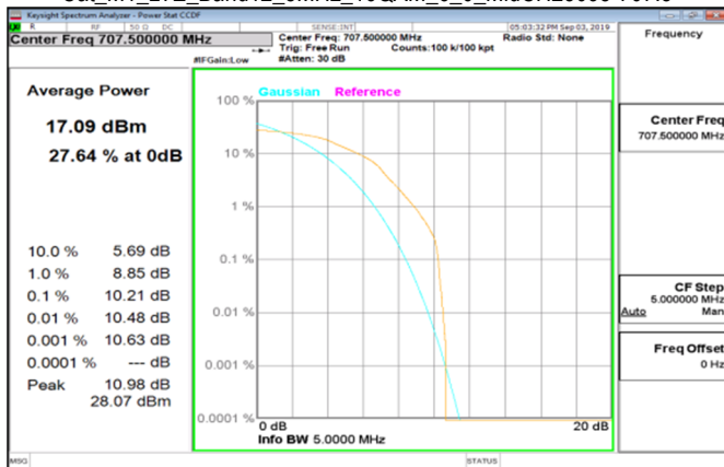
Cat_M1_LTE_Band12_5MHz_16QAM_6_0_MidCH23095-707.5
