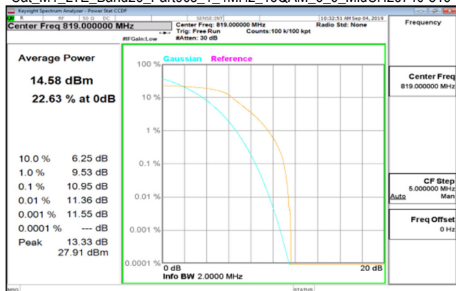
Cat M1 LTE_Band26_Part90s_1_4MHz_16QAM_6_0_MidCH26740-819
