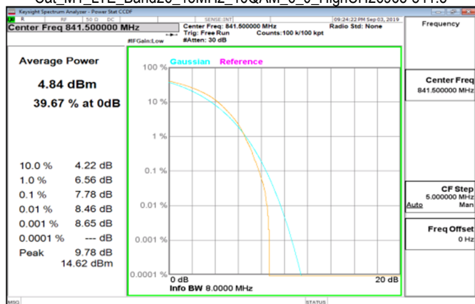
Cat M1 LTE_Band26_15MHz_16QAM_6_0_HighCH26965-841.5
