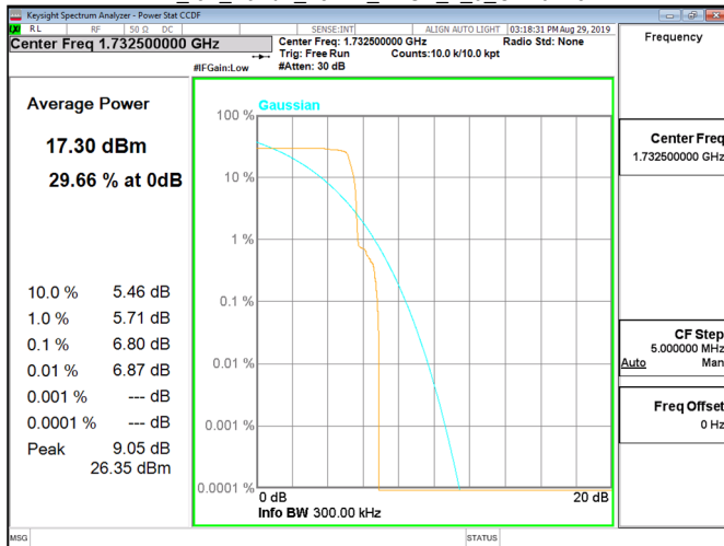
NB IoT_Band4_15kHz_BPSK_1_0_CH20399
