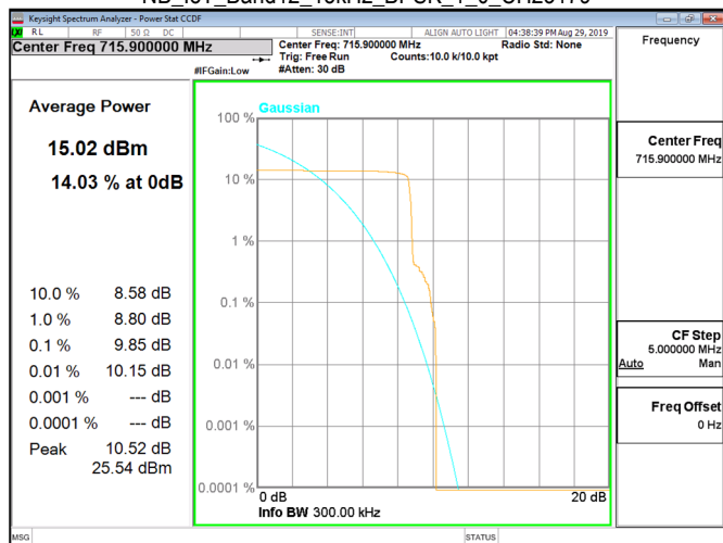
NB IoT_Band12_15kHz_BPSK_1_0_CH23179
