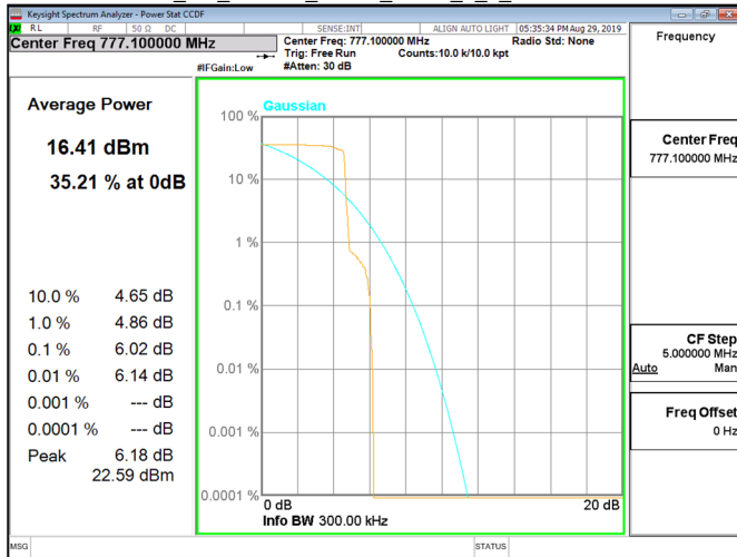
NB_IoT_Band13_15kHz_BPSK_1_0_CH23230
