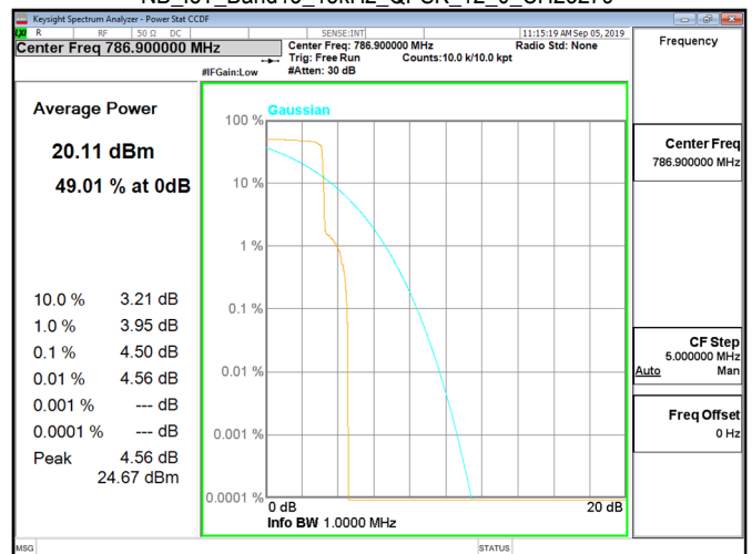
NB_IoT_Band13_15kHz_QPSK_12_0_CH23279
