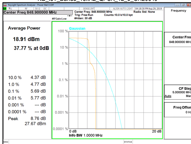
NB_IoT_Band5_15kHz_QPSK_12_0_CH20649
