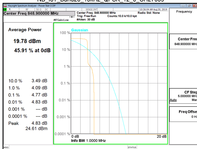
NB IoT_Band26_15kHz_QPSK_12_0_CH27039
