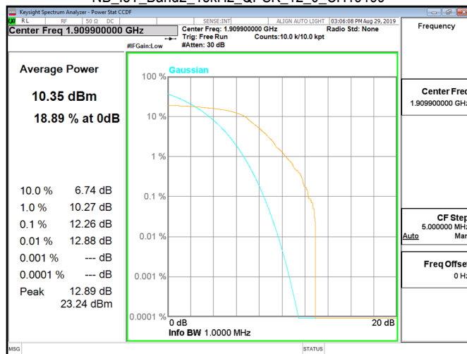
NB_IoT_Band2_15kHz_QPSK_12_0_CH19199
