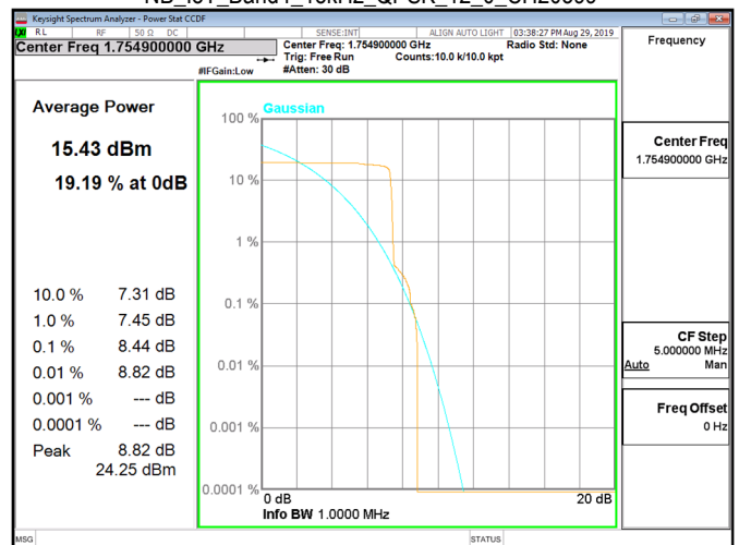
NB IoT_Band4_15kHz_QPSK_12_0_CH20399
