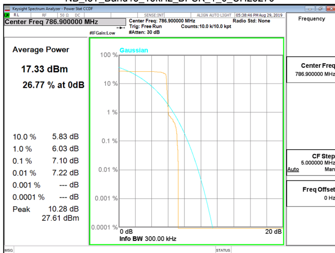
NB_IoT_Band13_15kHz_BPSK_1_0_CH23279
