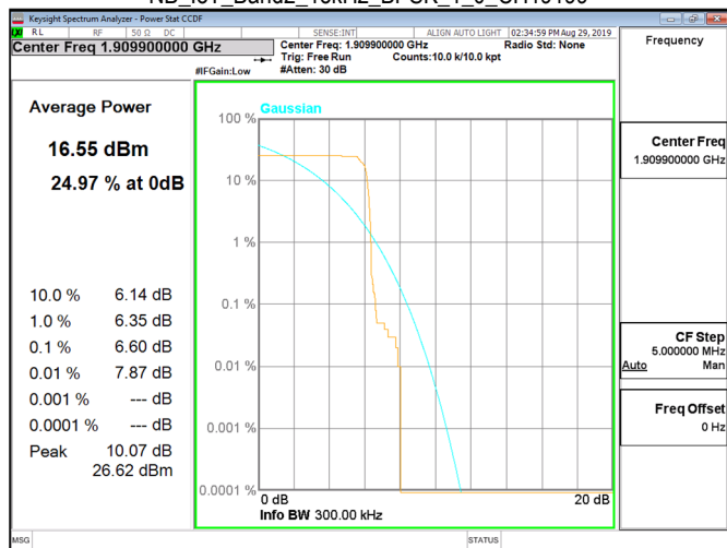
NB_IoT_Band2_15kHz_BPSK_1_0_CH19199
